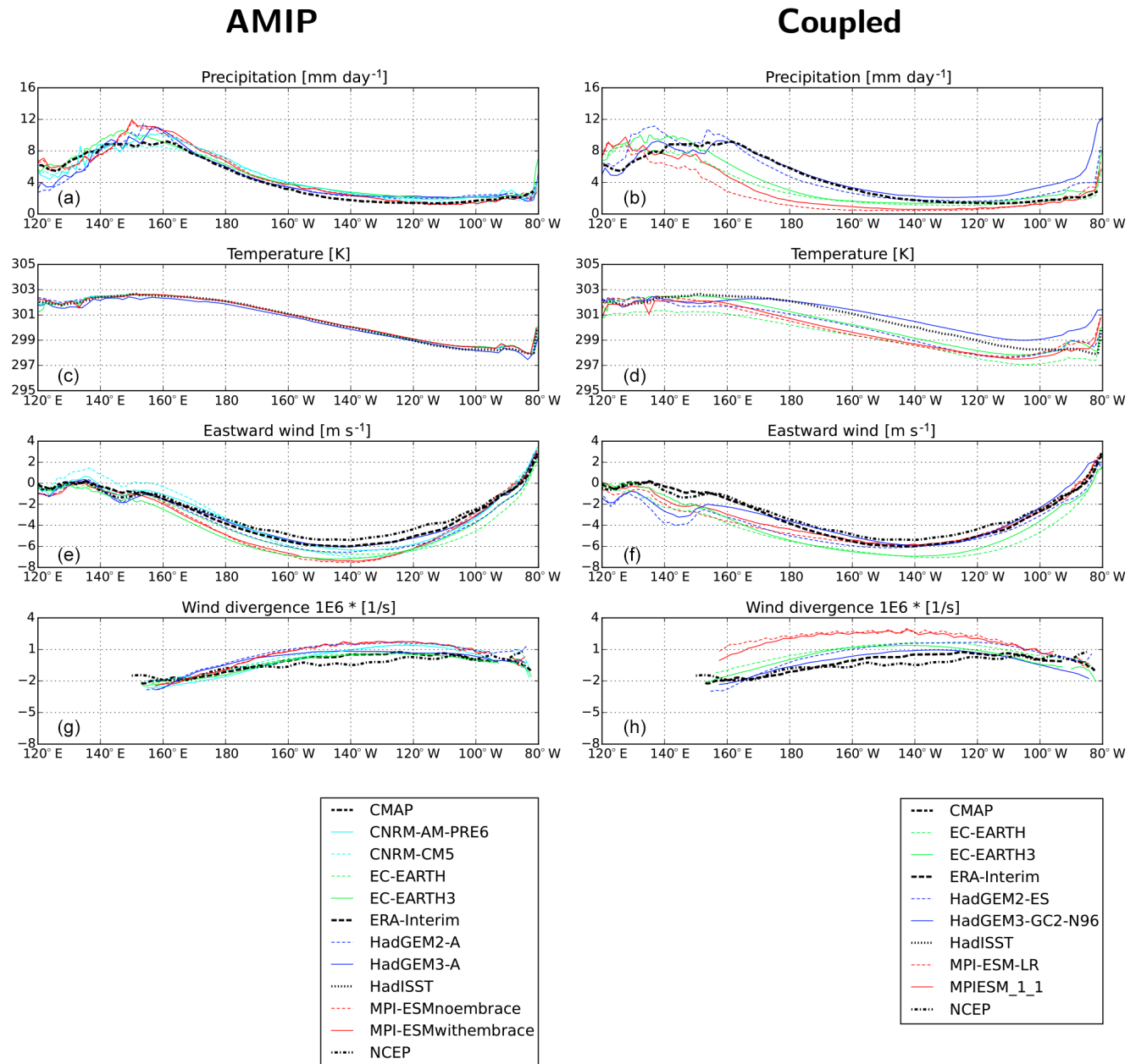
Figure 15. Equatorial mean ( 2.5^{\circ} N to 2.5^{\circ} S) values from top to bottom panels: precipitation, SST, 1000 hPa zonal wind speed, and total 925 hPa wind divergence averaged over the years 1982–2002 (MPI AMIP models 1979–1999). Values are plotted for the equatorial Pacific between 120^{\circ} E and 80^{\circ} W. The left column panels show model results from the AMIP simulations, the right column panels from the coupled (historical) simulations in comparison with observations.
