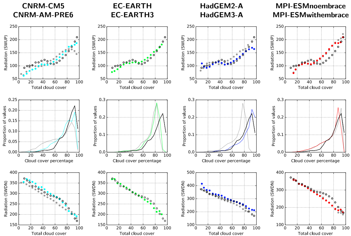
Figure 17. Top row panels: scatter plot of monthly mean TOA SWUP versus total cloud cover for the Southern Ocean region 30–65° S and season DJF averaged over the years 1986–2005 (MPI models 1980–1999, HadGEMs 1985–2004). Bottom row panels are the same for surface SWDN. Middle row shows fractional occurrence of monthly mean cloud cover over this region. Cloud observations are MODIS-L3 (2003–2014) and SWUP and SWDN are from CERES-EBAF (2001–2014). The EMBRACE-updated AMIP models are plotted in color, the corresponding CMIP5 models are shown in gray, and observations are in black. No radiation data from EC-Earth are available.
