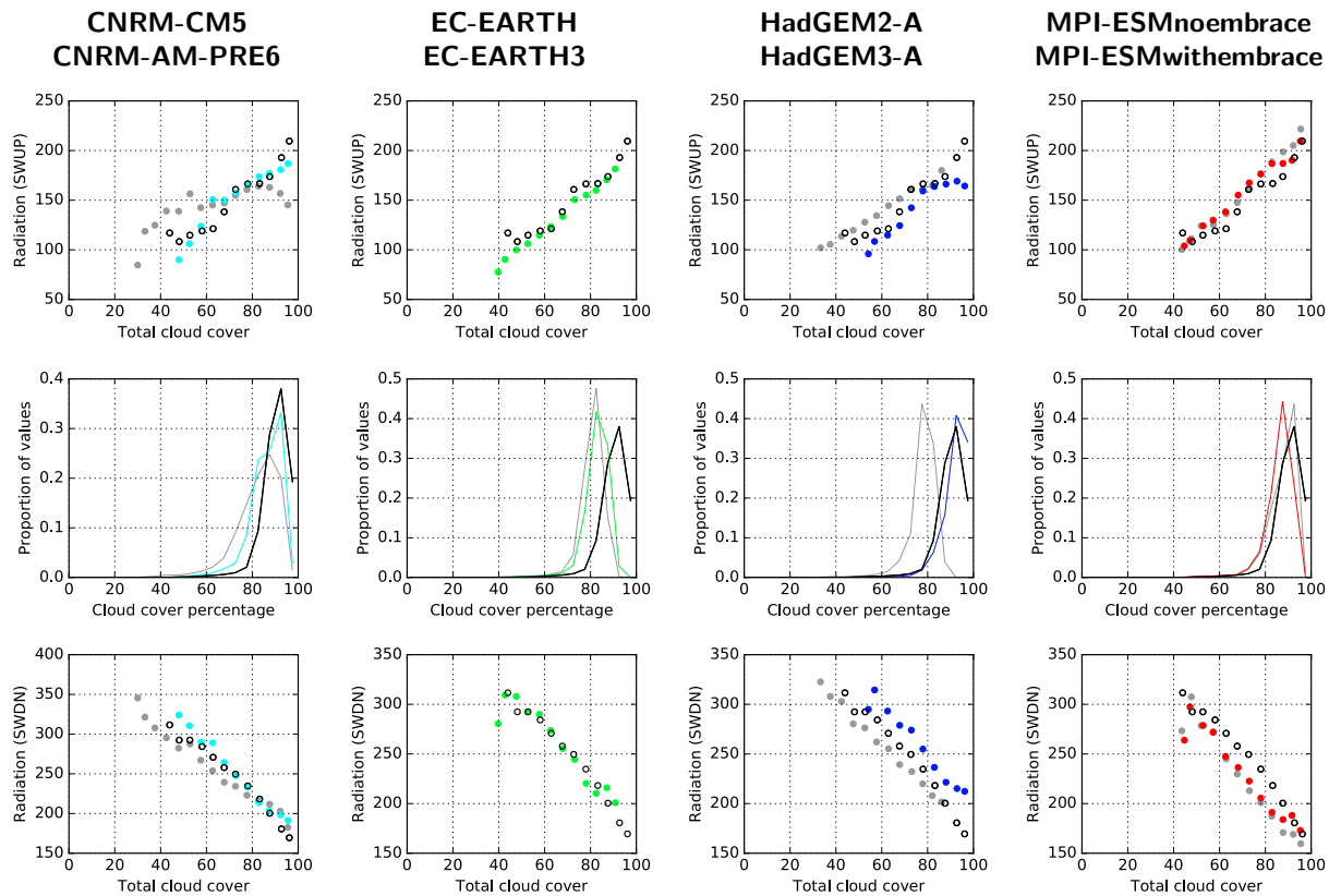
Figure 19. As Fig. 17 but for the southern part of the Southern Ocean region (SOC-S, 50–65° S).
