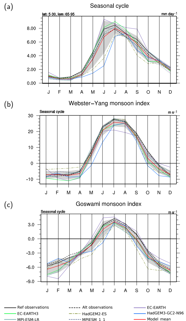
Figure 6. Mean annual cycle plots averaged over the years 1986–2005 (HadGEM: 1986–2004): (a) precipitation spatially averaged over 5–30° N, 65–95° E, (b) Webster and Yang monsoon index, (c) Goswami monsoon index. Shown are the coupled (historical) simulations. The reference observations (a) TRMM-L3 and (b, c) ERA-Interim are shown as solid black lines, the alternative observations (a) GPCP-SG and (b, c) NCEP 1 as black dashed lines.
