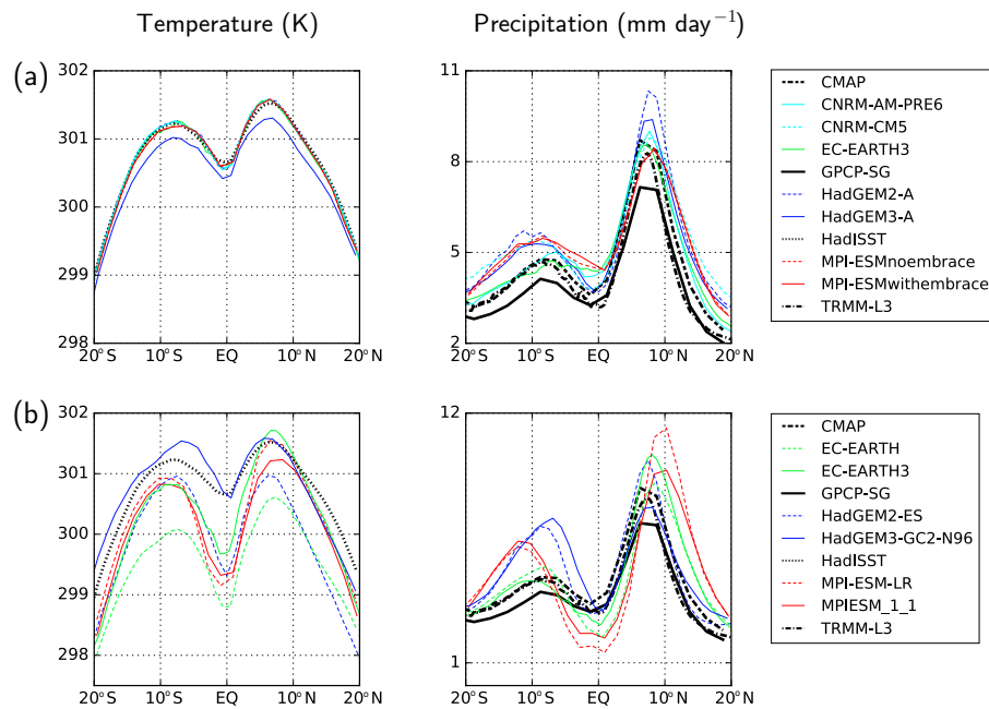
Figure 14. Latitude cross section of DJF SST in K (left column panels) and precipitation in mm per day (right column panels from (a) the AMIP simulations and (b) the coupled (historical) simulations in comparison with observations (HadISST for SST and CMAP, GPCP, and TRMM for precipitation). Values are zonal means averaged over all ocean grid cells in the longitude band 120° E to 100° W and averaged over the years 1982–2002 (MPI AMIP models 1979–1999).
