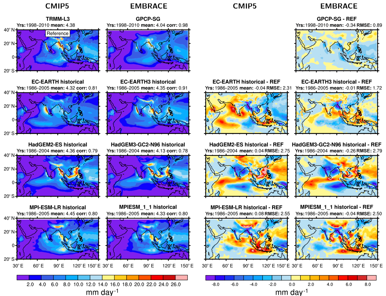
Figure 3. Leftmost two columns: seasonal mean precipitation for JJAS from observations (TRMM, GPCP) and the coupled simulations. The years used to calculate the averages shown are given above each panel (“yrs”). Rightmost two columns: differences relative to TRMM. Columns 1 and 3 show the original CMIP5 model versions, columns 2 and 4 the EMBRACE-updated models. The domain-averaged annual mean (“mean”), linear pattern correlation (“corr”; leftmost two columns), mean bias (“mean”), and root mean square error (RMSE; rightmost two columns) compared with TRMM are given above the individual panels.
