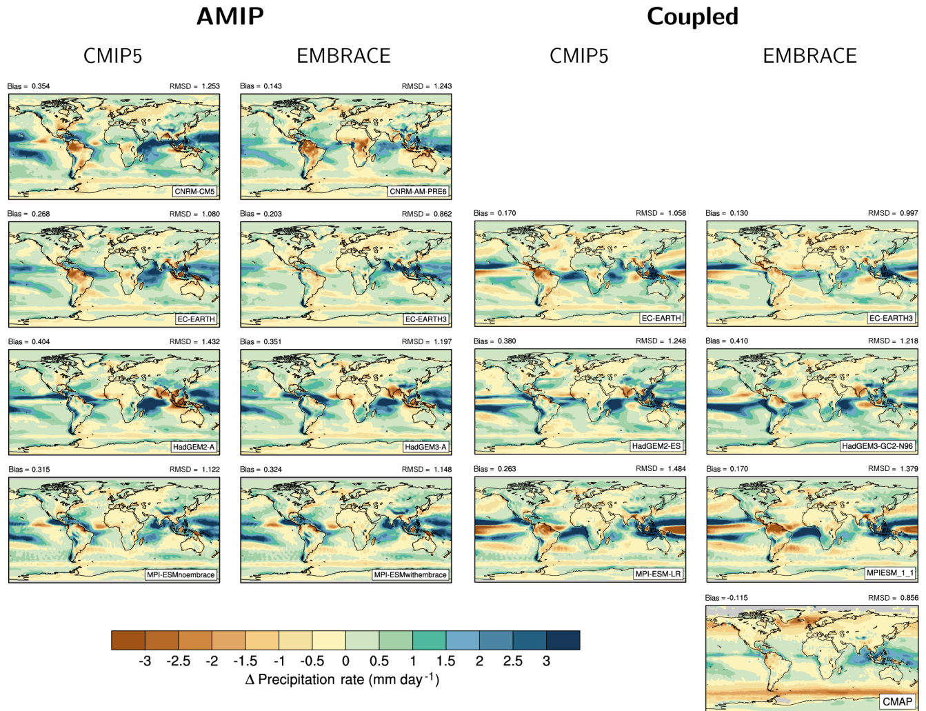
Figure 2. Bias in annual mean precipitation rate ( \text{mm day}^{-1} ) for the 20-year period 1986–2005 (MPI AMIP models: 1980–1999) as the difference between the Global Precipitation Climatology Project (GPCP) and from left to right (1) the AMIP simulations from the CMIP5 models, (2) the corresponding EMBRACE models, (3) the coupled historical simulations from the CMIP5 models, and (4) the corresponding EMBRACE models. Data from CMAP are shown as a second reference dataset in the lowermost rightmost panel. The global averaged annual mean bias (“bias”) and root mean square deviation (RMSD) compared with GPCP are given above the individual panels.
