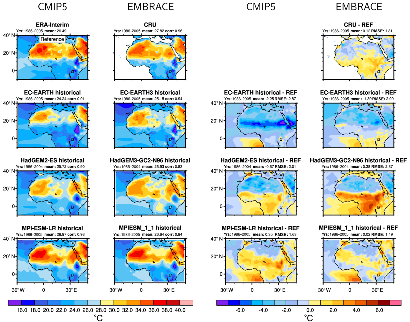
Figure 8. Leftmost two columns: seasonal mean 2 m temperature for JJAS from reanalysis data (ERA-Interim), the CRU dataset, and the coupled simulations averaged over the years 1986–2005 (HadGEM: 1986–2004). Rightmost two columns: differences relative to ERA-Interim. Columns 1 and 3 show the original CMIP5 model versions, columns 2 and 4 the EMBRACE-updated models. The domain-averaged annual mean (“mean”), linear pattern correlation (“corr”; leftmost two columns), mean bias (“mean”; rightmost two columns) compared with ERA-Interim are given above the individual panels.
