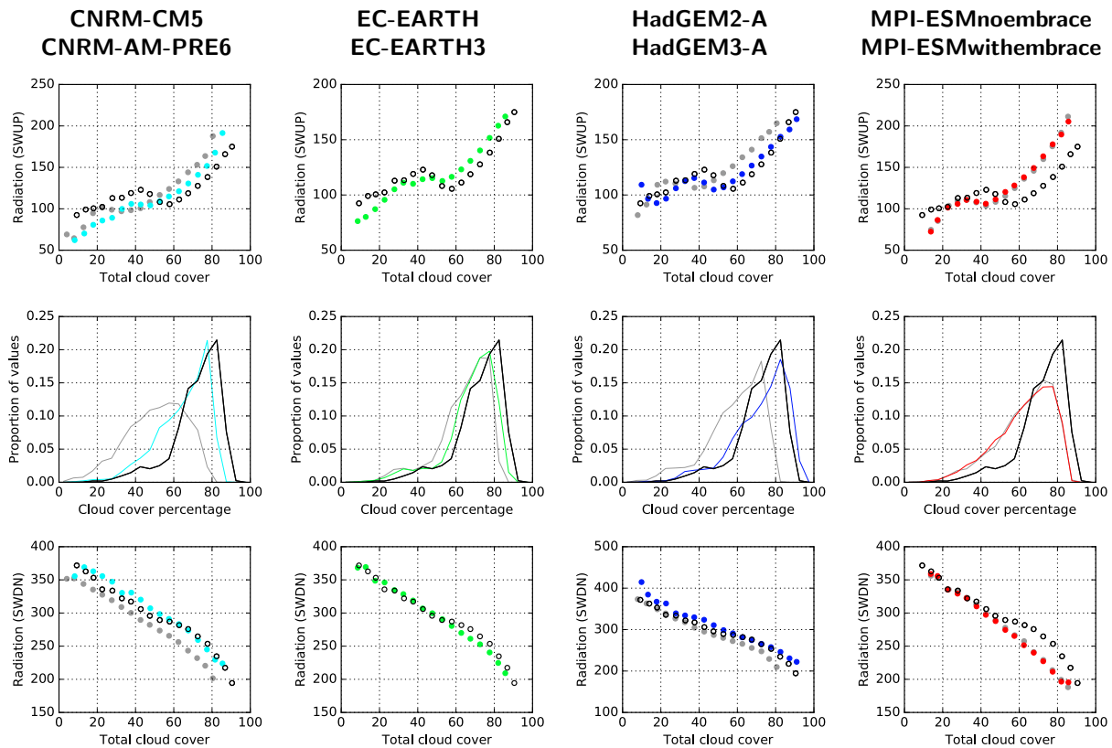
Figure 18. As Fig. 17 but for the northern part of the Southern Ocean region (SOC-N, 30–45° S).
