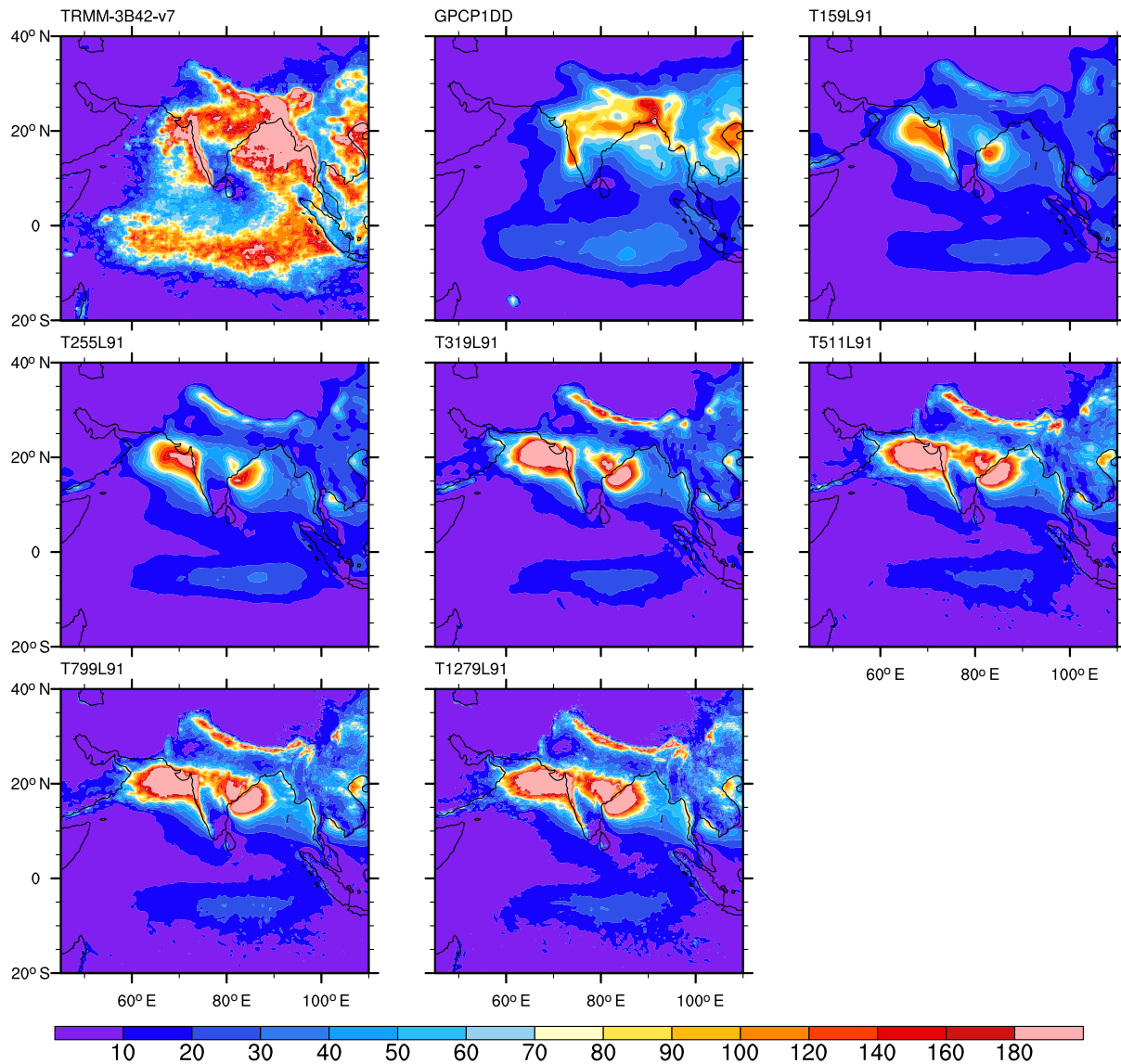
Figure 13. The 3–10 day band-pass-filtered JJAS precipitation variance for TRMM ( 0.25^\circ \times 0.25^\circ ), GPCP-1DD ( 1^\circ \times 1^\circ ), and the T159, T255, T319, T511, T799, and T1279 EC-Earth simulations ( \text{mm}^2 \text{day}^{-2} ).
