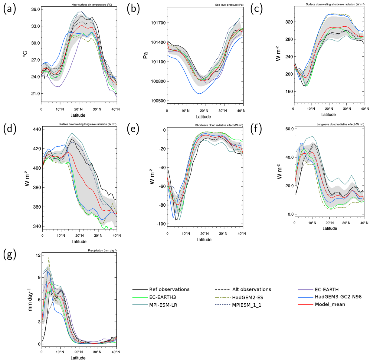
Figure 10. The 10^{\circ} W– 10^{\circ} E zonal average JJAS mean values averaged over the years 1986–2005 (HadGEM: 1986–2004) as a function of latitude ( x axis) for (a) 2 m temperature, (b) sea level pressure, (c) surface downwelling solar radiation, (d) surface downwelling longwave radiation, (e) shortwave cloud radiative forcing, (f) longwave cloud radiative forcing, and (g) precipitation. Model results are for the coupled simulations. The reference observations (a, b) ERA-Interim, (c–f) CERES-EBAF, and (g) TRMM-L3 are shown as solid black lines, the alternative observations (a) CRU, (f) SRB, and (g) GPCP-SG as black dashed lines. The gray shading shows the inter-model standard deviation.
