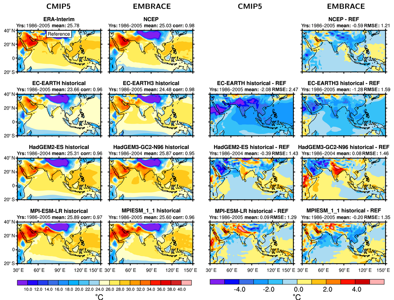
Figure 4. Leftmost two columns: seasonal mean 2 m temperature for JJAS from reanalysis data (ERA-Interim), the NCEP 1 dataset, and the coupled simulations averaged over the years 1986–2005 (HadGEM: 1986–2004). Rightmost two columns: differences relative to ERA-Interim. Columns 1 and 3 show the original CMIP5 model versions, columns 2 and 4 the EMBRACE-updated models. The domain-averaged annual mean (“mean”), linear pattern correlation (“corr”; leftmost two columns), mean bias (“mean”), and root mean square error (RMSE; rightmost two columns) compared with ERA-Interim are given above the individual panels.
