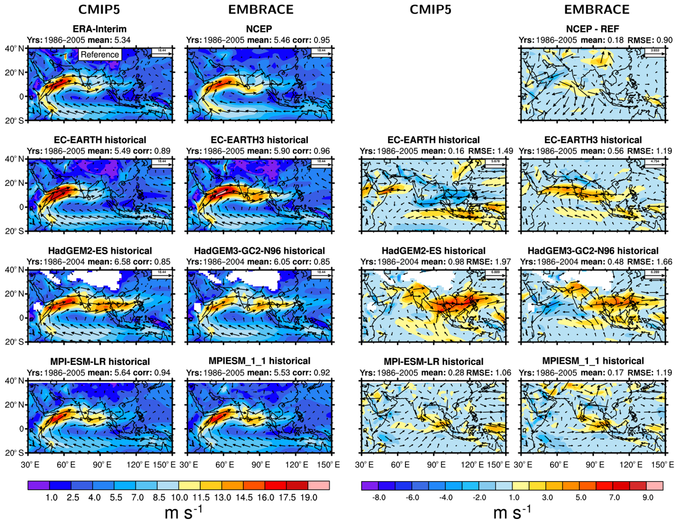
Figure 5. Leftmost two columns: seasonal mean zonal wind speed at 850 hPa for JJAS from reanalysis data (ERA-Interim, NCEP 1) and the coupled simulations averaged over the years 1986–2005 (HadGEM: 1986–2004). Rightmost two columns: differences relative to ERA-Interim. Columns 1 and 3 show the original CMIP5 model versions, columns 2 and 4 the EMBRACE-updated models. The domain-averaged annual mean (“mean”), linear pattern correlation (“corr”; leftmost two columns), mean bias (“mean”), and root mean square error (RMSE; rightmost two columns) compared with ERA-Interim are given above the individual panels.
