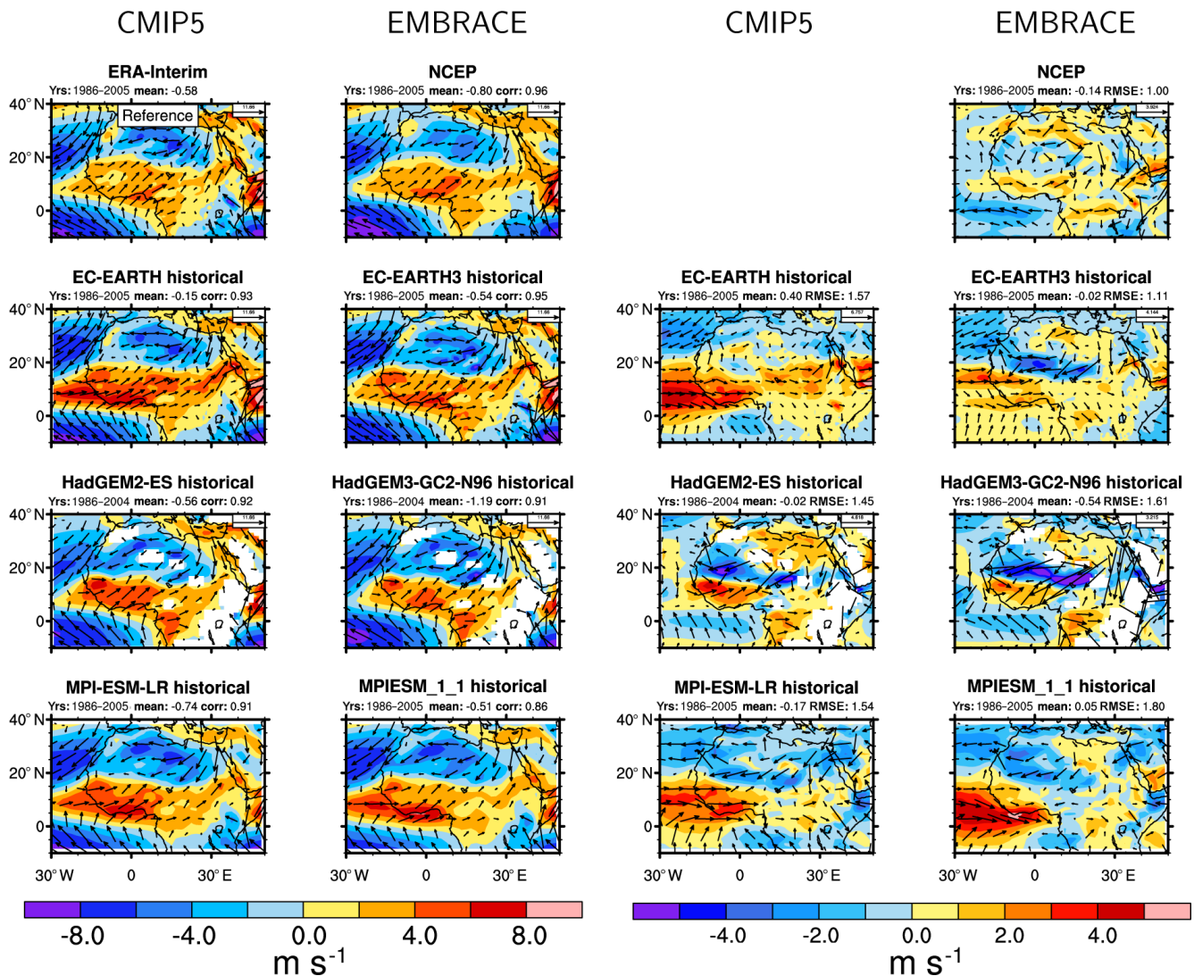
Figure 9. Leftmost two columns: seasonal mean wind speed at 925 hPa for JJAS from reanalysis data (ERA-Interim and NCEP 1) and the coupled simulations averaged over the years 1986–2005 (HadGEM: 1986–2004). Rightmost two columns: differences relative to ERA-Interim. Columns 1 and 3 show the original CMIP5 model versions, columns 2 and 4 the EMBRACE-updated models. The domain-averaged annual mean (“mean”), linear pattern correlation (“corr”; leftmost two columns), mean bias (“mean”), and root mean square error (RMSE; rightmost two columns) compared with ERA-Interim are given above the individual panels.
