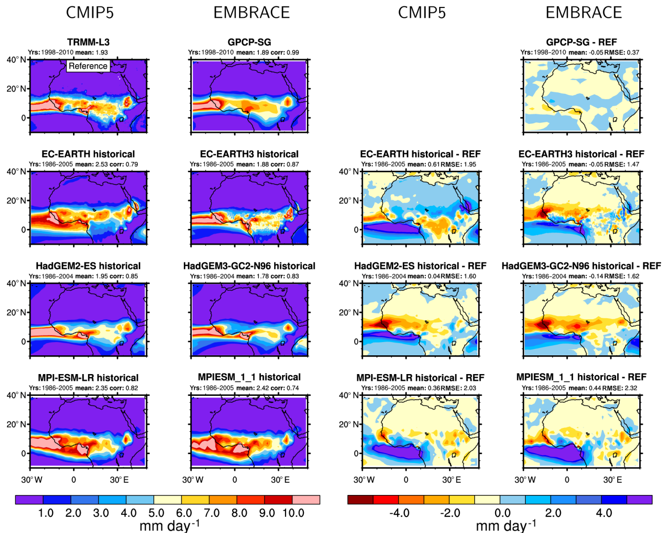
Figure 7. Leftmost two columns: seasonal mean precipitation for JJAS from observations (TRMM, GPCP) and the coupled simulations. The years used to calculate the averages shown are given above each panel (“yrs”). Rightmost two columns: differences relative to TRMM. Columns 1 and 3 show the original CMIP5 model versions, columns 2 and 4 the EMBRACE-updated models. The domain-averaged annual mean (“mean”), linear pattern correlation (“corr”; leftmost two columns), mean bias (“mean”), and root mean square error (RMSE; rightmost two columns) compared with TRMM are given above the individual panels.
