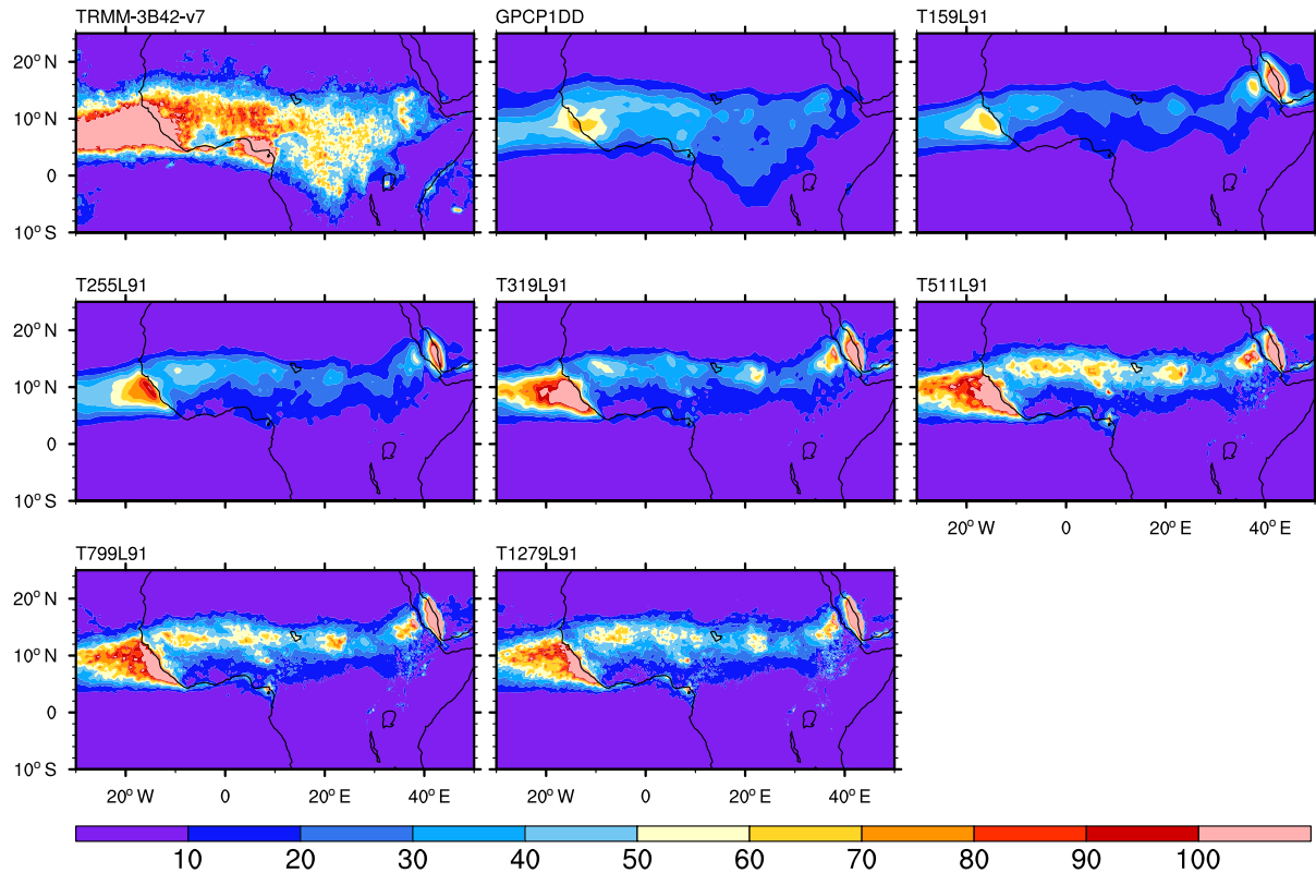
Figure 12. The 3–10-day band-pass-filtered JJAS precipitation variance for TRMM ( 0.25^\circ \times 0.25^\circ ), GPCP-1DD ( 1^\circ \times 1^\circ ), and T159, T255, T319, T511, T799, and T1279 EC-Earth simulations ( \text{mm}^2 \text{day}^{-2} ).
