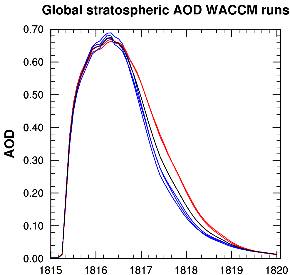
Figure 8: Global stratospheric mean AOD of the 5 CESM-WACCM ensemble runs. Easterly phase nudged QBO forcing is used from the observed strength starting with 1982 for two runs (red), and from the observed strength starting with 1991 for three runs (blue). The ensemble mean of the five runs is in black. Vertical dotted line marks date of injection of SO 2 .
