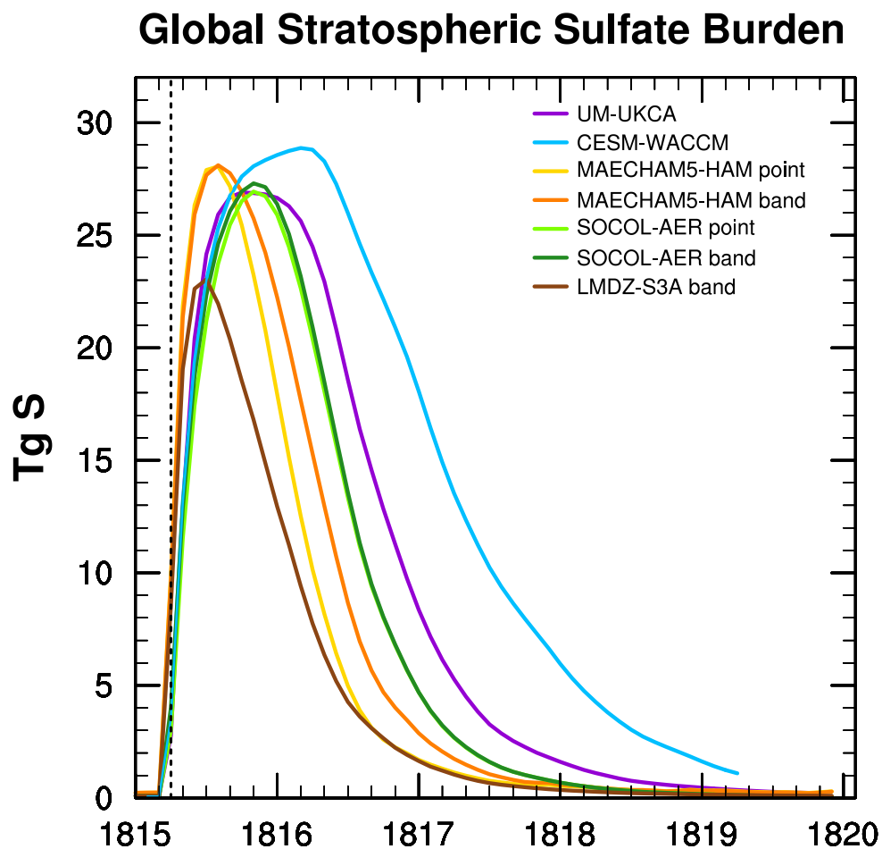
Figure 2: Global stratospheric burden of \text{SO}_4 in TgS vs time. Vertical dashed black line indicates month of injection.
