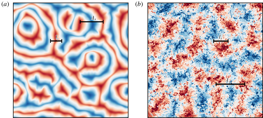
FIGURE 1. Temperature fields in the midplane for two different Rayleigh numbers with Pr=1 and aspect ratio 24. Red indicates hot rising fluid, and blue cold descending fluid. (a) Close to onset in the weakly nonlinear regime, regular patterns with wavelength \lambda_s emerge. (b) Connected large-scale structures are present in the turbulent regime as well, and their length scale \lambda_s is increased compared to onset. The small-scale fluctuations can be removed with a filter of width l_s , which preserves the large-scale rolls. For similar visualizations of turbulent superstructures, see also Hartlep et al. (2005), Stevens et al. (2018) and Pandey et al. (2018).
