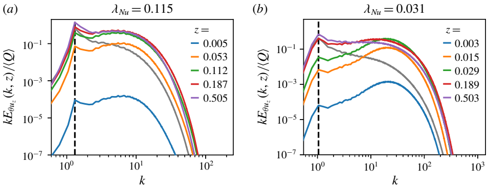
FIGURE 12. Pre-multiplied spectra, kE_{\theta u_z}(k, z) , for (a) Ra = 1.02 \times 10^5 and (b) Ra = 1.07 \times 10^7 , and different heights z . The height-averaged spectrum is shown in dark grey. The thermal boundary layer thickness \lambda_{Nu} is given for reference. A peak at the same position k is present at all heights, also in the boundary layer, characterizing the size of the superstructure. However, close to the boundary layer a second maximum emerges. This is related to small-scale fluctuations. The maximum at small scales is highlighted through the presentation in pre-multiplied form.
