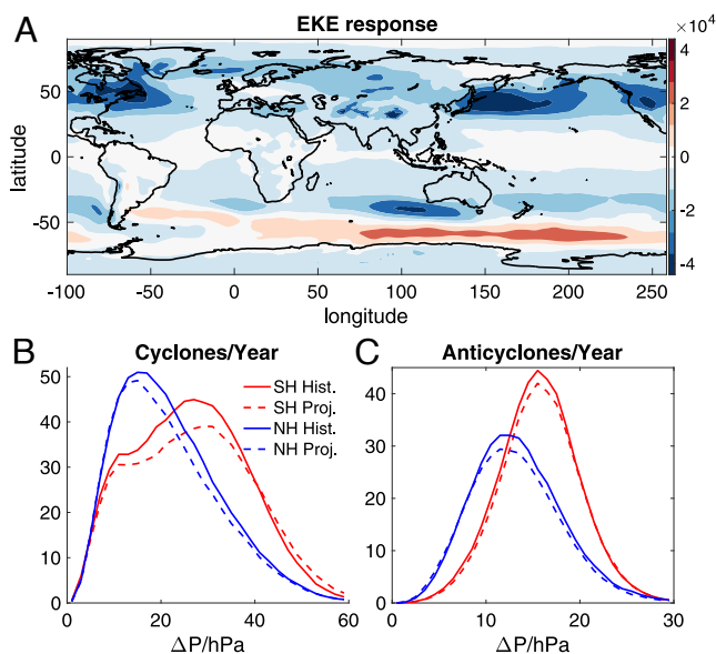
Fig. 4. (A) Response of baroclinic activity ( \text{hPa}^2 ) to climate change. Baroclinic activity is defined as in Fig. 1B. The response is defined as the change in climatology between the projected and historical simulations ( Materials and Methods ). (B and C) The probability distribution function of cyclone and anticyclone intensity for the NH and SH (blue and red, respectively) for the historical and projected runs (solid and dash lines, respectively).
