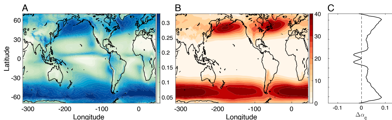
Fig. 1. (A) Climatology of cloud-albedo. (B) Climatology of synoptic scale activity, defined as E = \overline{\text{SLP}^2} , where the bar stands for the time mean and the prime is defined as the high-pass of zonal wavenumbers above five of the sea-level pressure (SLP). (C) The hemispheric difference (SH minus NH) in zonal mean cloud-albedo as a function of latitude. The cloud-albedo is calculated from CERES short-wave flux data, following the method presented in (1). Data for A and C is the daily mean data from CERES and data for B is taken from ERA5, as described in Materials and Methods .
