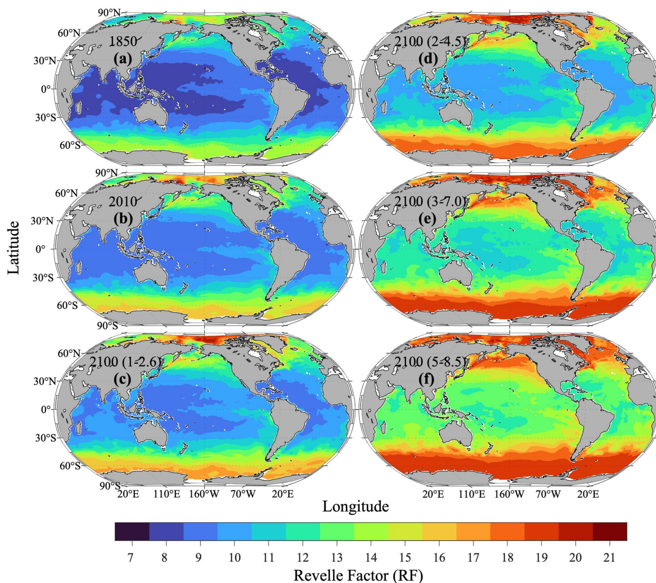
Figure 9. Surface ocean Revelle Factor (RF, inter-model median) in the decades around (a) 1850, (b) 2010, (c) 2100 (SSP1-2.6), (d) 2100 (SSP2-4.5), (e) 2100 (SSP3-7.0), and (f) 2100 (SSP5-8.5). SSP is short for Shared Socioeconomic Pathway.
