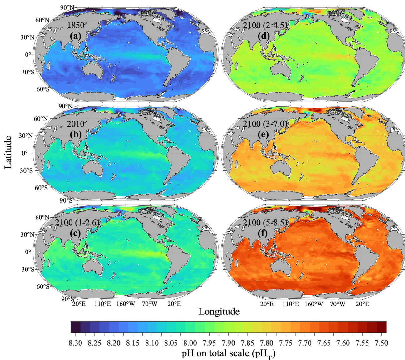
Figure 7. Surface ocean pH on total scale ( \text{pH}_T , inter-model median) in the decades around (a) 1850, (b) 2010, (c) 2100 (SSP1-2.6), (d) 2100 (SSP2-4.5), (e) 2100 (SSP3-7.0), and (f) 2100 (SSP5-8.5). SSP is short for Shared Socioeconomic Pathway.
