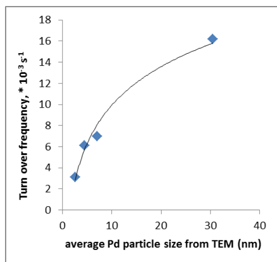
Figure 3. Effect of palladium particle size on turn-over-frequency for nitrite reduction over Pd supported CNF-Ni foam estimated based on TEM analysis.
