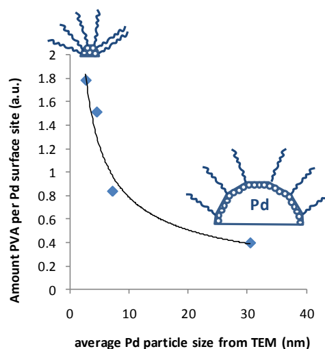
Figure 4. Amount of PVA per palladium surface site calculated from Table 1 together with a pictorial view for the smallest and the largest palladium particles.
