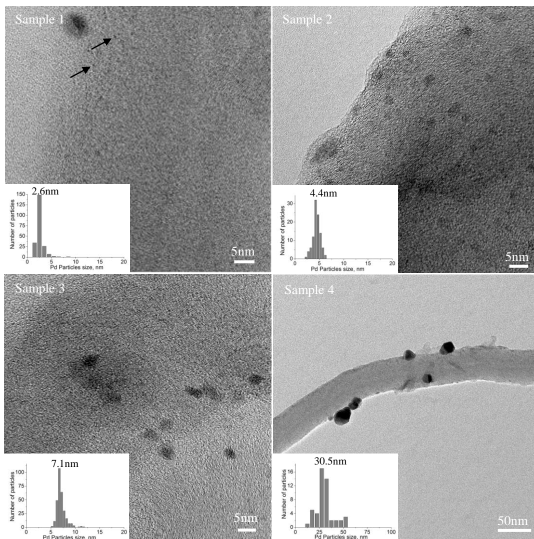
Figure 1. TEM images and respective histograms of palladium particle size distribution deposited on Hairy foam samples 1-4.
