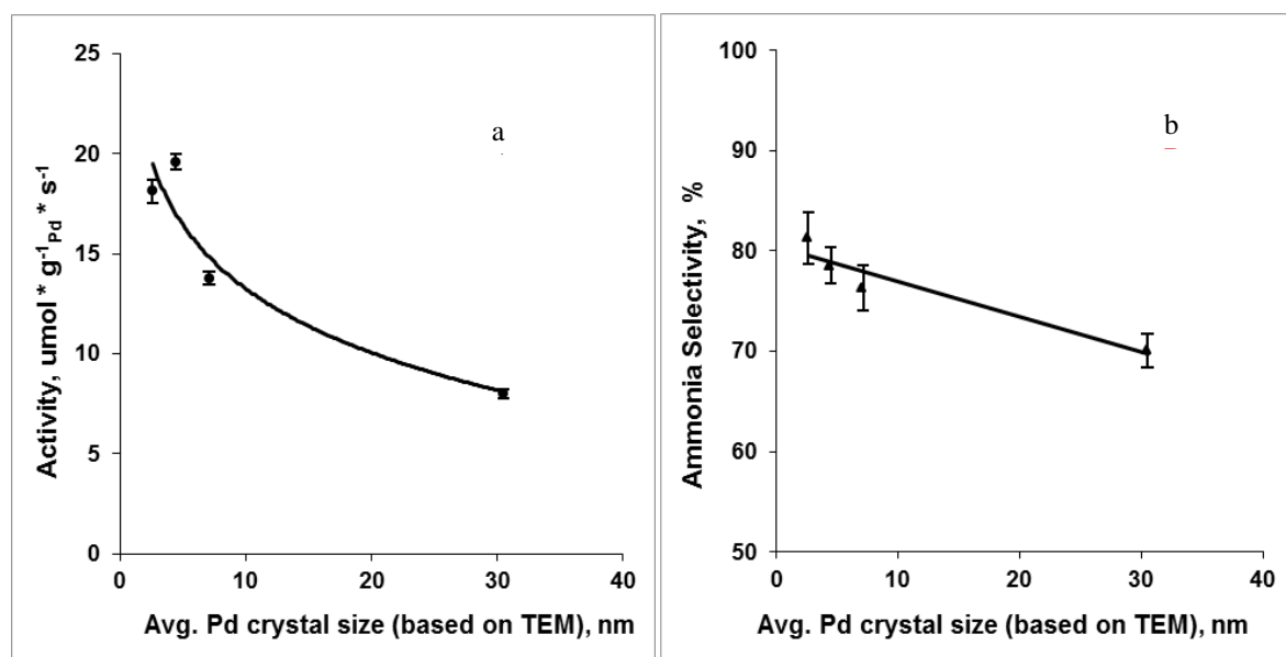
Figure 2: Influence of the Pd particle size on the activity per gram of palladium (a) and ammonia selectivity (b) during nitrite reduction for Pd supported CNF-Ni foam.
