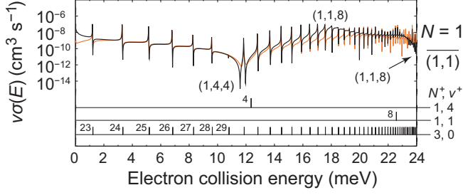
FIG. 5. (Color online) Calculated N = 1 contribution to the MQDT local rate coefficient v\sigma_{\text{DR}}(\varepsilon) for the DR of \text{HD}^+(^2\Sigma_g^+, v_i^+ = 0) in N_i^+ = 1 and illustration of the validation for the assignment of low- n resonances. Black line: full result for N = 1 ; red (gray) line: result obtained on eliminating the excitation channel (N^+, v^+) = (1, 1) as symbolically indicated in the right margin. The resonances are labeled using the notation of Fig. 3.
