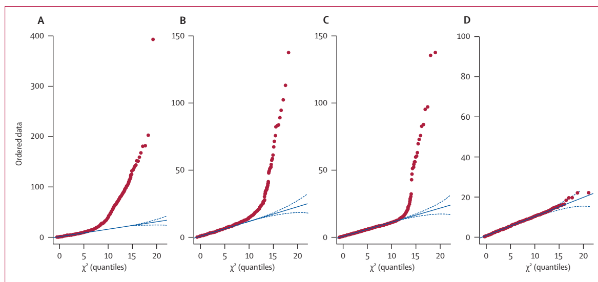
Figure 2: QQ (quartile–quartile) plots of different stages of quality control
