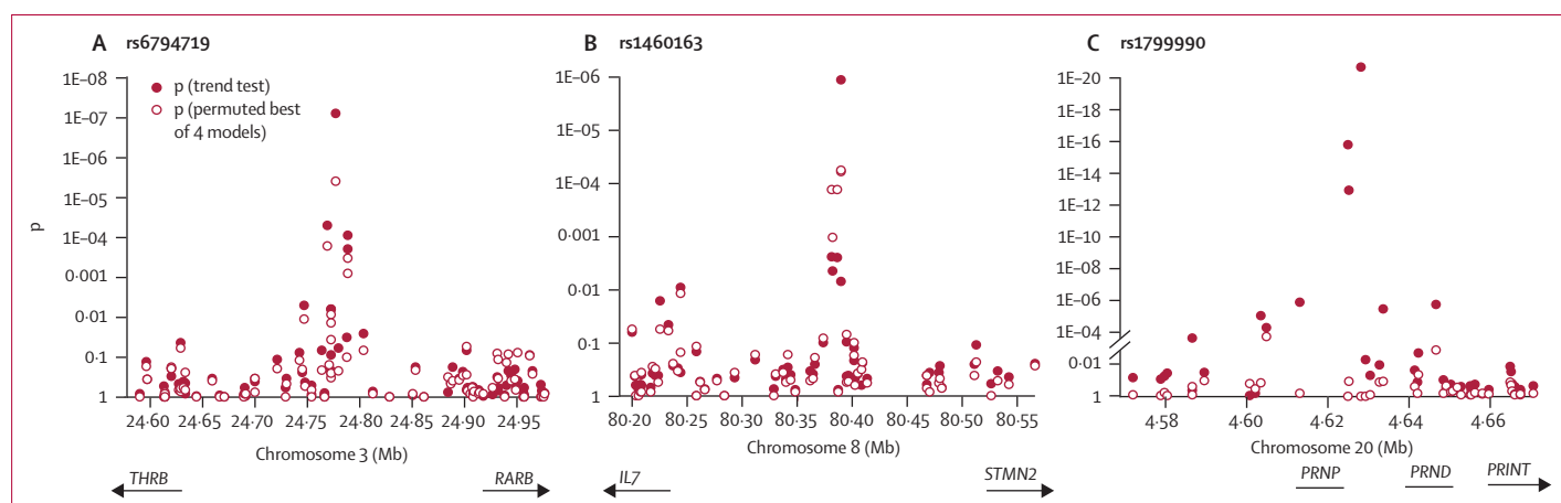
Figure 3: Physical location and p of allelic test and best of four genetic models
