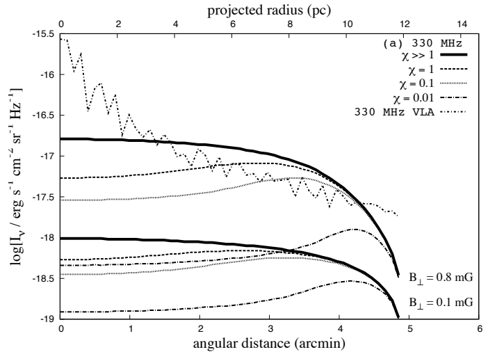
FIG. 4.— Comparison of the actual emission intensity as a function of angular distance from the center of Sgr B2 and that expected from models of synchrotron emission from secondary electrons at 330 MHz. The curves are for the parameters labelled and match those of Figure 9 of POE08 .
