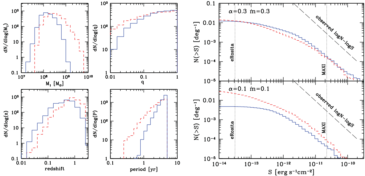
Figure 6. Left-hand plot: properties of the PTA-MBHB population observable through periodicity, contributing at a level of 0.1 ns or more to the PTA signal in the 3 \times 10^{-9} to 10^{-6} Hz frequency window in our default model, averaged over 100 Monte Carlo realizations. Systems with orbital periods < 5 yr only were selected. From the top left to the bottom right, we plot the primary mass, mass ratio, redshift and period distributions. Right-hand plot: periodic MBHB contribution to the X-ray \log N - \log S function, assuming a bolometric correction of 30 (0.5–10 keV). The top panel is for our default model; the bottom panel is for a less optimal model ( \dot{m} = 0.1 ) for which MBHB–disc decoupling occurs earlier. Vertical dotted lines depict the flux limit for a single eROSITA pointing and for the combined pointings of MAXI over one month. Dashed thin line depicts the upper end of the AGN \log N - \log S as observed by ROSAT (Voges 1999). In both plots, line style is as in Fig. 1.
