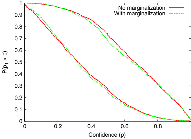
FIG. 5 (color online). Comparison of performance of model selection when including the total number of events as a parameter of the model (labeled “no marginalization”) and when this parameter is marginalized over (labeled “with marginalization”). The small difference indicates that the total number of events contains relatively little information compared to the shape of the parameter distributions. We show the same model comparison as in Fig. 4.
