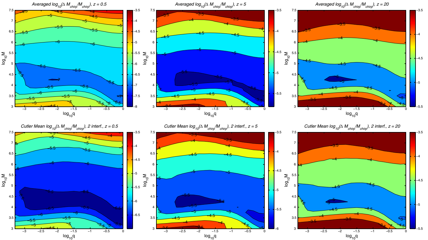
FIG. 15 (color online). Contours of the error on the chirp mass in the (M, q) plane at different redshifts (from left to right: z = 0.5, 5 and 20 ). The top row refers to the averaged code, the bottom row to the Cutler code with T_{\text{obs}} = 3 yrs and two interferometers.
