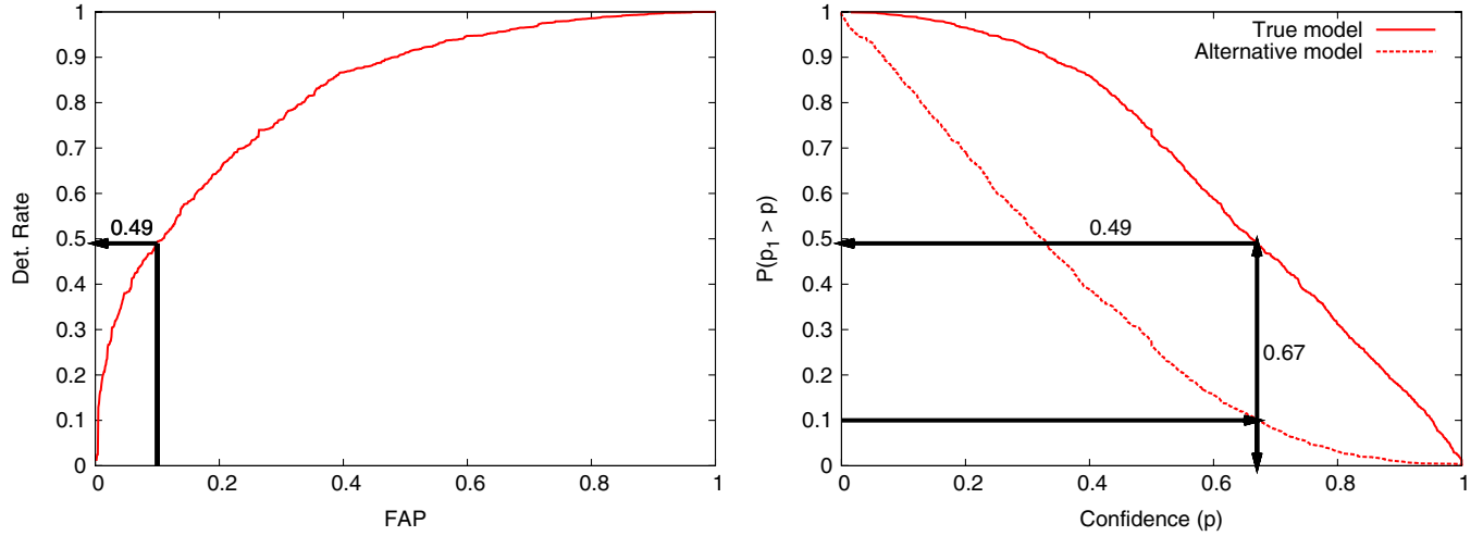
FIG. 4 (color online). Two alternative ways to represent our ability to distinguish models. The left panel shows an ROC curve, while the right panel shows the CDF of the confidence achieved over multiple realizations of the correct (upper curve) and wrong (lower curve) model. More details are given in the text. The model comparison used for this figure was VHM-noZ-Edd-co to VHM-noZ-Edd-ch , for a three-month LISA observation and the most pessimistic assumption ( T_2 ) on the transfer function.
