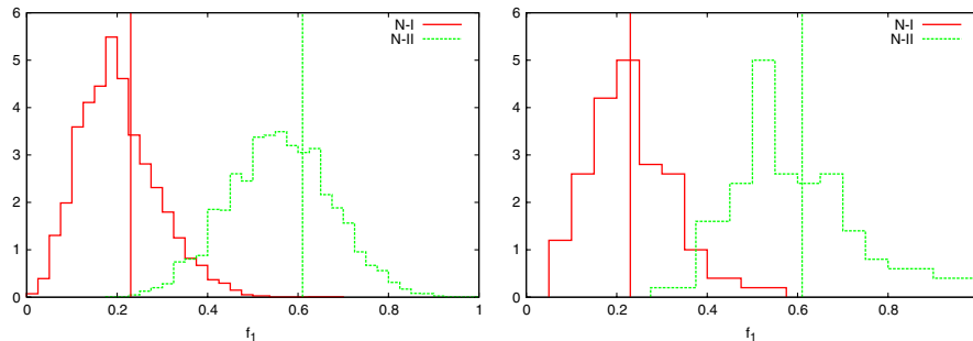
FIG. 10 (color online). Summary of the model mixing results for models \mathcal{N} -I and \mathcal{N} -II. In both panels, the horizontal axis shows the mixing fraction for model VHM-noZ-Edd-co . The left panel shows the posterior probability distribution function for this mixing fraction as found in one particular realization of each model. The right panel shows how the peak of the posterior was distributed over 100 different realizations of each of the two models. The vertical lines show the true values of the mixing fraction.
