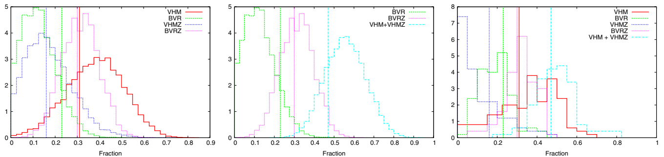
FIG. 11 (color online). Summary of model mixing results for model \mathcal{N} -III. We show the mixing fraction of the given model on the horizontal axis. The left panel shows the posterior probability distribution of the mixing fraction for each of the four models, VHM , BVR , VHM-Z and BVR-Z , found when analyzing a single realization of model \mathcal{N} -III. The central panel shows the same thing, but now considering the fractions of BVR , BVR-Z and the sum VHM+VHM-Z in the mixed model. The right panel shows the distribution of the peak of the posterior pdf found over 100 different realizations of the \mathcal{N} -III model.
