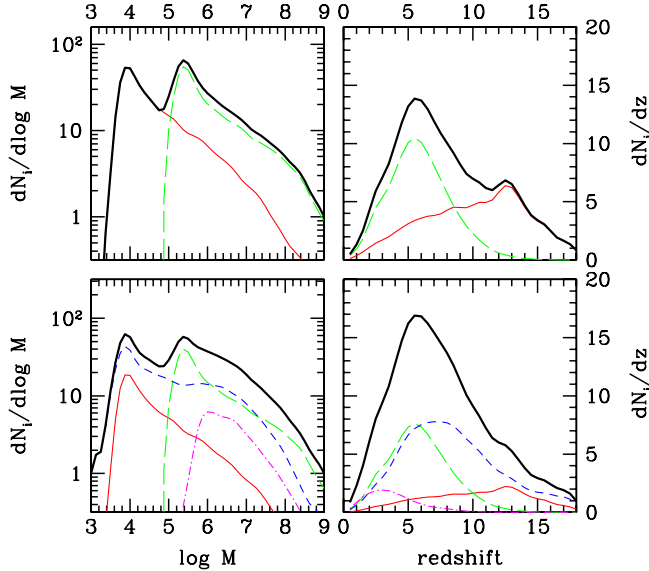
FIG. 9 (color online). Examples of mixed models. In the upper panels we show marginalized dN_i/dM (left) and dN_i/dz (right) distributions for the model \mathcal{N} -I (thick solid black lines), in which we mix models VHM-noZ-Edd-co (thin solid red line) and BVR-noZ-Edd-co (thin long-dashed green line). The relative contribution of the models is given by Eq. (19) with f_1 = 0.23 , f_3 = 0.77 (cf. Table II). In the lower panels we show the same distributions for the model \mathcal{N} -IV (thick solid black lines) in which we mix four “pure” models. The thin lines represent the relative contribution of the individual models VHM-noZ-Edd-co (solid red), VHM-Z-Edd-co (short-dashed blue), BVR-noZ-Edd-co (long-dashed green), and BVR-Z-Edd-co (dot-dashed magenta). The relative contribution of the models is given again by Eq. (19) with f_1 = 0.08 , f_3 = 0.22 , f_5 = 0.56 and f_7 = 0.14 (cf. Table II).
