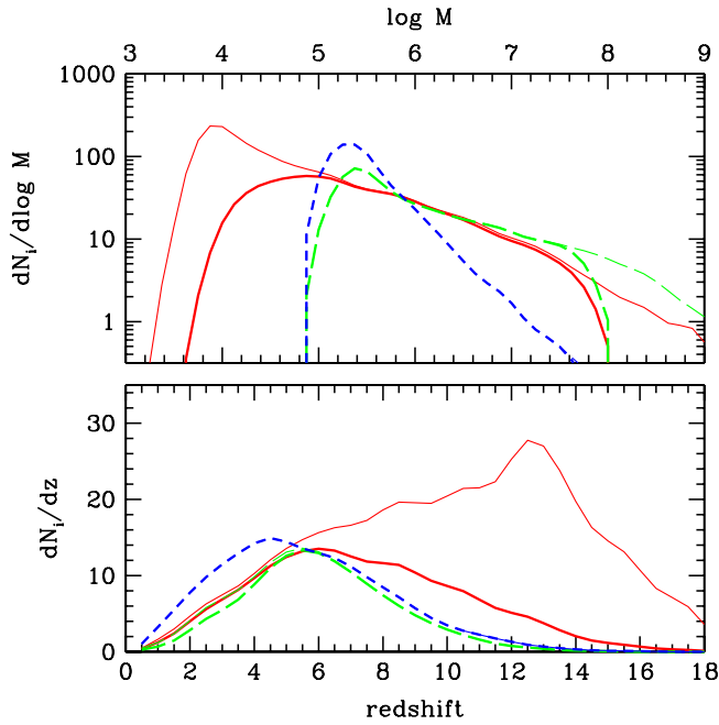
FIG. 2 (color online). Examples of the marginalized distributions dN_i/dM (upper panel) and dN_i/dz (lower panel) predicted by different MBH formation models. In each panel we plot the following models: VHM-noZ-Edd-co (solid red lines); BVR-noZ-Edd-ch (long-dashed green lines); BVR-noZ-MH-co (short-dashed blue lines). Thin lines represent the coalescence distributions predicted in three years, while thick lines represent the theoretically observable distributions after the transfer function T_3(z, M, q) has been applied, namely, N_{T_{i,3}}(M) and N_{T_{i,3}}(z) (see text for details).
