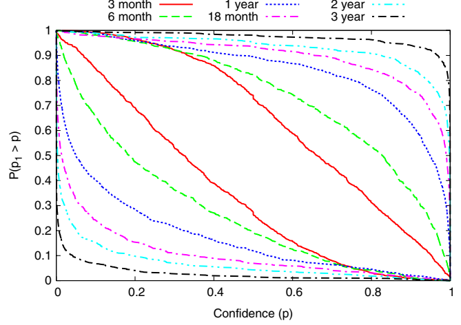
FIG. 8 (color online). Effect of the LISA observation duration on the pure model selection results. We compare VHM-noZ-Edd-co and VHM-noZ-Edd-ch , under the most pessimistic choice ( T_2 ) for the transfer function.
