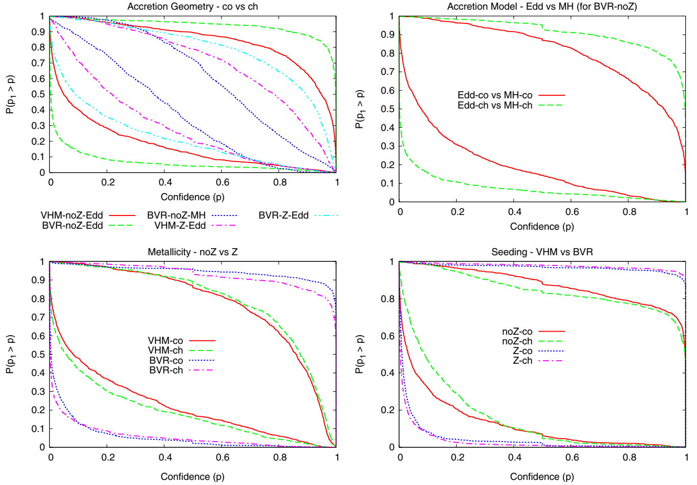
FIG. 6 (color online). Results for comparisons of the pure models. Each plot shows all possible comparisons varying only one of the elements listed in Table I. Top left panel: we consider the effect of the accretion geometry , comparing coherent to chaotic for each of the combinations of the other ingredients. Top right panel: we consider the effect of the accretion model , comparing Eddington accretion to Merloni-Heinz accretion for the BVR-noZ models. Bottom left: we consider the effect of metallicity by comparing the noZ to Z models for VHM-co , VHM-ch , BVR-co and BVR-ch . Bottom right: we consider the effect of the seeding assumption, comparing the VHM to BVR models for the four combinations noZ-co , noZ-ch , Z-co and Z-ch , each with Eddington accretion. In all panels we are making the most pessimistic assumptions about the detector, i.e., we use the transfer function T_2 (one interferometer, \rho_{\text{thr}} = 20 ). These results are for a 3 month LISA observation, except for the top left panel which is for a 1 yr observation.
