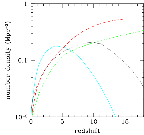
FIG. 17 (color online). Comoving number density of MBHs in the four formation models we have considered. Solid curve: BVR-Z. Dotted curve: BVR-noZ. Short-dashed curve: VHM-noZ. Long-dashed curve: VHM-Z.
