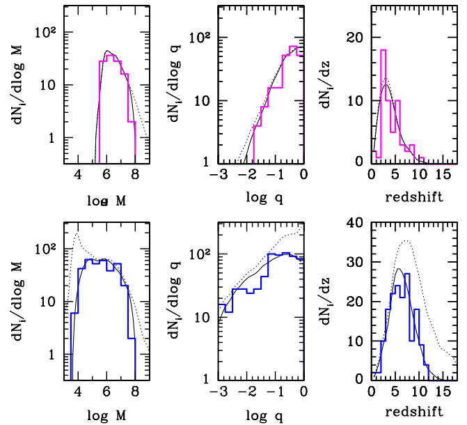
FIG. 3 (color online). Examples of Monte Carlo generated data sets. The left panels show the dN_i/dM distributions, the central panels show the dN_i/dq distributions and the right panels show the dN_i/dz distributions. The upper panels refer to model BVR-Z-Edd-co , the lower panels to model VHM-Z-Edd-co . In each panel the dotted curves represent the theoretical distributions, and the solid curves represent the theoretically observable distribution filtered with the transfer function T_3 . The thick histograms show one Monte Carlo realization of the theoretical distribution, as observed by LISA, under the assumption of two operational interferometers and \rho_{\text{thr}} = 8 .
