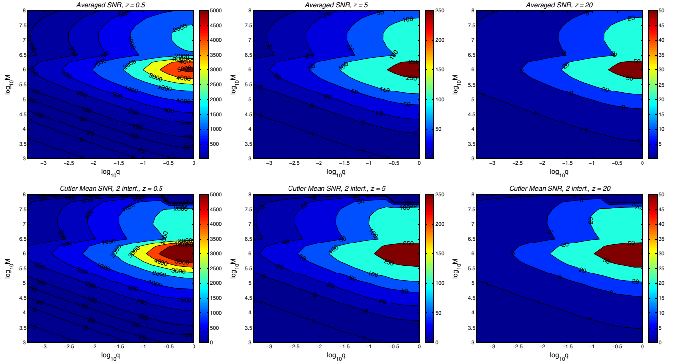
FIG. 14 (color online). SNR contours in the (M, q) plane at different redshifts (from left to right: z = 0.5, 5 and 20 ). The top row refers to the averaged code, the bottom row to the Cutler code with T_{\text{obs}} = 3 yrs and two interferometers.
