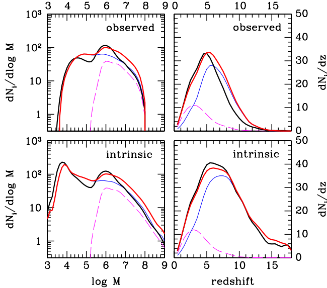
FIG. 13 (color online). Comparison of intrinsic and “recovered” distributions for the consistently mixed models. In each panel, the thick solid black curve shows the intrinsic distribution of mergers in the model, the red solid line shows the “recovered” distribution, which is a sum of the VHM-Z and BVR-Z models, weighted by the best-fit mixing parameter. The thin lines show the contributions to this recovered distribution from the VHM-Z (solid blue) and BVR-Z (dashed magenta) models. The left panels show the distributions of the masses of mergers, while the right panels show the distributions of the redshifts of mergers. The upper panels show the distribution for observed merger events, while the lower panels show the intrinsic distribution of mergers.
