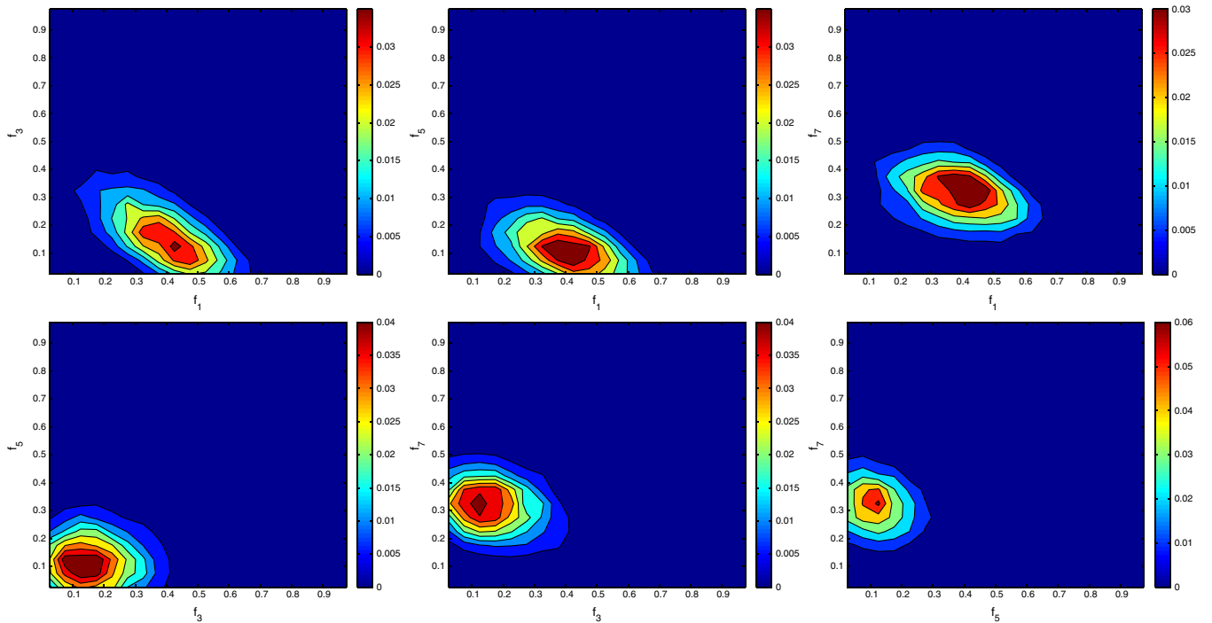
FIG. 12 (color online). Two-dimensional marginalized posterior PDFs obtained from a single realization of model \mathcal{N} -III. Each plot shows the mixing fraction of one model component against the mixing fraction of a second component. The models are numbered from 1, 3, 5 and 7, corresponding to VHM , VHM-Z , BVR and BVR-Z respectively, as in Table I. The top row shows comparisons between model 1 (horizontally) and models 3, 5 and 7, respectively. The bottom row shows comparisons 3 to 5, 3 to 7 and 5 to 7, respectively. Note that the individual components of VHM and VHM-Z are poorly constrained, which is why the plots involving VHM models have larger correlation contours than the BVR to BVR-Z comparison (bottom right).
