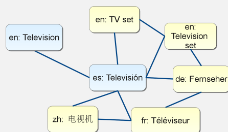
Figure 4.9: Misleading graph topology
