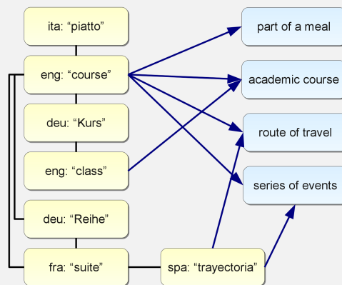
(b) Input graph G_0 including translations
