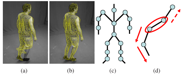
Figure 3. Although local optimization is prone to errors, often only a single branch of the kinematic chain is affected (a). This reduces the computational burden for global optimization since it can be performed in a lower dimensional subspace to correct the estimation error (b). After detecting misaligned limbs (red circle), the kinematic chain is traversed (red arrows) to label bones and associated joints that have to be globally optimized (c,d).
