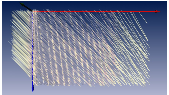
(b) Stream lines of p correspond to the path lines in v .
