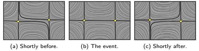
Figure 4: Saddle connection bifurcation.
