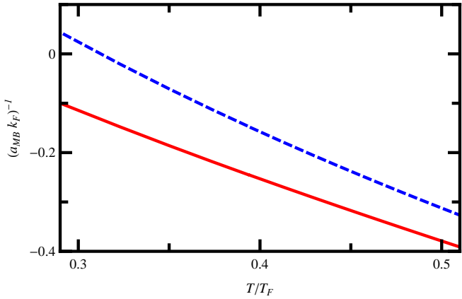
FIG. 3: Bare many-body scattering length a_{\text{MB}}^{\text{B}} (dashed line) and fully renormalized many-body scattering length a_{\text{MB}}^{\infty} (full line) as a function of temperature T in the unitarity limit for the balanced Fermi gas. The Fermi wavevector k_{\text{F}} and Fermi temperature T_{\text{F}} are directly related to the total particle density through the Fermi energy \epsilon_{\text{F}} = k_{\text{B}}T_{\text{F}} = \hbar^2 k_{\text{F}}^2/2m = \hbar^2(3\pi^2 n)^{2/3}/2m , which is calculated with the RG approach. The many-body scattering length is inversely proportional to the Cooper-pair chemical potential, and the difference between the bare and the renormalized value is due to the repulsive Cooper-pair interaction effects.
