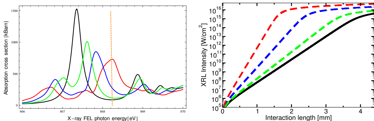
Figure 6.12.: (a) The absorption cross section is shown for the field-free case in black and for laser-dressing with an optical laser intensity of 10^{12} W/cm 2 in green, 3 \times 10^{12} W/cm 2 in blue and 7 \times 10^{12} W/cm 2 in red. The dotted, orange line denotes the x-ray FEL central frequency \omega_{\text{XFEL}} . (b) The XRL's intensity is shown as a function of the interaction length for the scenarios of the same color in (a).
