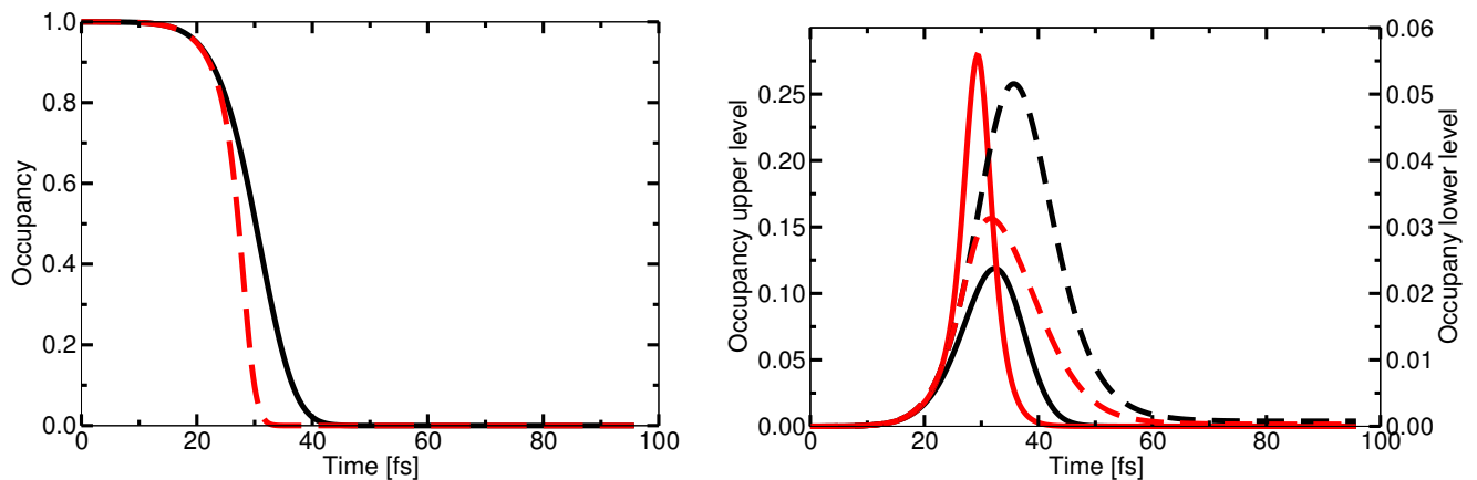
Figure 6.7.: (a) Ground state occupancy at z = 0 without (black) and with (dashed, red) optical laser dressing. (b) The upper state occupancy at z = 0 is shown with the solid lines without (black) and with (red) optical laser dressing respectively. The lower state occupancy at z = 0 is shown with the dashed lines without (black) and with (red) optical laser dressing respectively.
