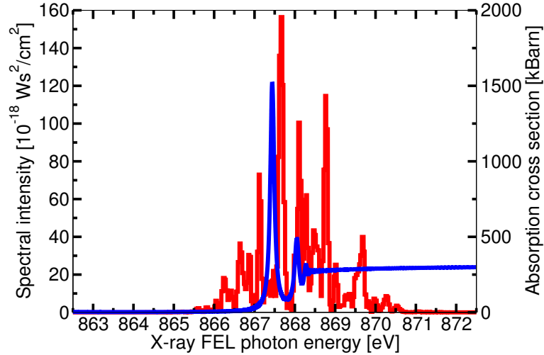
Figure 6.5.: Total photoionization cross section \sigma_N^{\text{Tot}}(\omega_{\text{XFEL}}) for neutral Ne without laser dressing (blue) and the spectral intensity S_P(\omega_X) of a random x-ray FEL pulse (red) with \omega_{\text{XFEL}} = 868.2\text{ eV} and \Delta\omega_{\text{XFEL}} = 2.6\text{ eV} .
