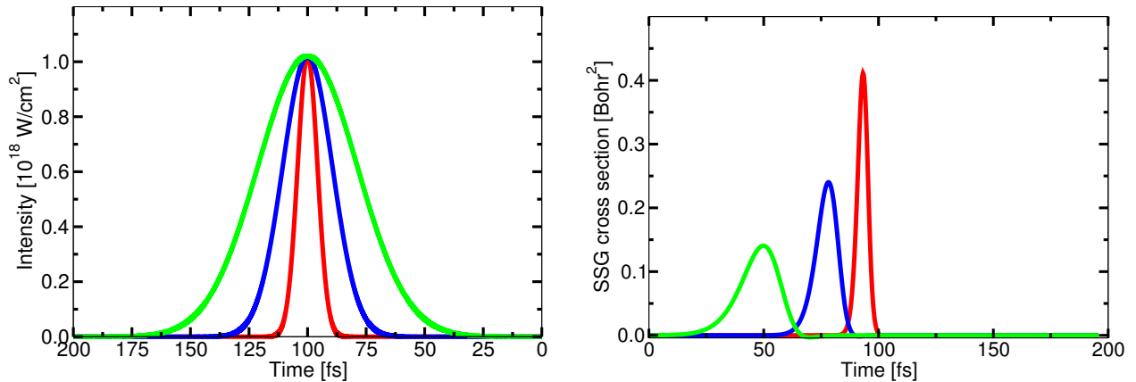
Figure 6.16.: (a) X-ray FEL pulses with FWHM 10 fs (red), 25 fs (blue) and 50 fs (green). In order to keep the peak intensity of the blue and green pulses at 10^{18} W/cm ^2 , the number of photons per pulse N_{\text{ph}} has been increased by a factor 2.5 and 5 for the 25 fs and 50 fs pump pulses, respectively. (b) SSG achieved by the pump pulses shown in (a) with the same colors.
