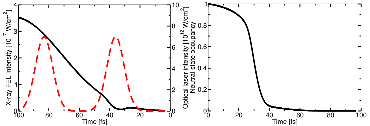
Figure 6.34.: Temporal profiles of the x-ray pump pulse with peak intensity of 3.5 \times 10^{17} W/cm ^2 (black line) and the optical laser pulse with twin-peaks (red line) are shown after a propagation distance of 3 mm. Based on the reshaping of the x-ray pump pulse it is evident that only the front portion of the pulse contributes to the excitation of the atoms. b) Temporal profile of the groundstate occupancy after 3 mm is displayed, confirming the conclusion from a) as all atoms are excited after 60 fs before the second optical laser peak arrives.
