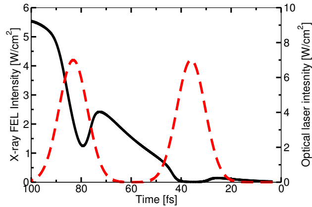
Figure 6.36.: Temporal profiles of the x-ray pump pulse with peak intensity of 5.6 \times 10^{16} \text{W/cm}^2 (black line) and the optical laser pulse with twin-peaks (red line) are shown after a propagation distance of 2.5 mm. Reshaping of the x-ray pump pulse due to absorption results in the loss of the initially chosen overlap with the optical laser pulse as the first 40 fs of the x-ray pulse are effectively gone.
