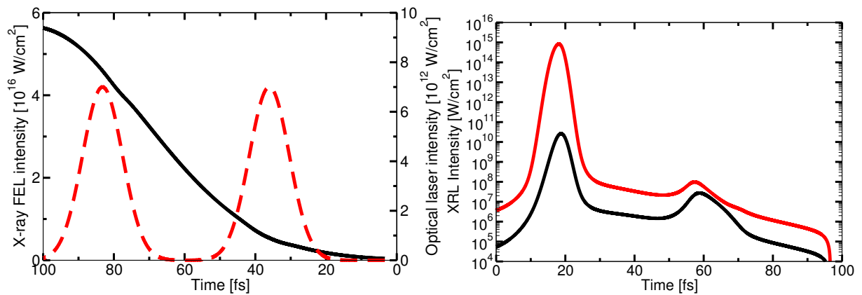
Figure 6.35.: Temporal profiles of the initial x-ray pump pulse with peak intensity of 5.6 \times 10^{16} W/cm ^2 (black line) and the optical laser pulse with twin-peaks (red line). b) The XRL pulse for laser-dressing with the twin-peak optical laser pulse from a) is displayed after a propagation distance of 0.5 mm (black line) and after a propagation distance of 4.4 mm (red line).
