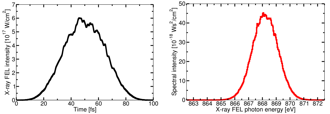
Figure 3.3.: Average intensity (left) and average spectral intensity (right) over 800 shots for SASE pulses with central frequency \omega_S = 868.2 eV, spectral FWHM \Delta\omega_S = 2.0 eV and average pulse duration \tilde{t}_P = 100 fs.
