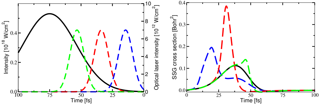
Figure 6.10.: Dependence of gain modulation on the optical laser's position. Red lines illustrate the ideal case. (a) X-ray FEL pump pulse (black line) and optical laser pulses (colored dashed lines) at different positions. (b) XRL's SSG for the field-free case (black line) and for the case with laser-dressing (colored dashed lines) for different positions of the optical laser pulse relative to the x-ray FEL pulse.
