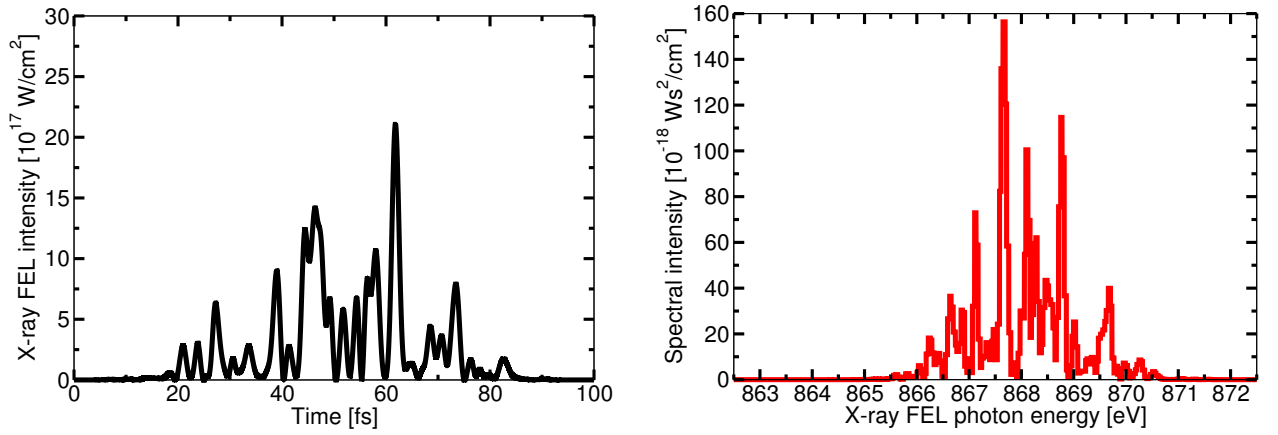
Figure 3.2.: Intensity (left) and spectral intensity (right) for a single SASE pulse with central frequency \omega_S = 868.2 eV, spectral FWHM \Delta\omega_S = 2.0 eV and average pulse duration \tilde{t}_P = 100 fs.
