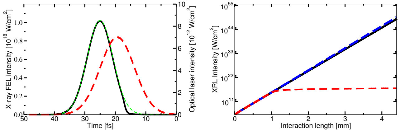
Figure 6.20.: (a) The final x-ray FEL pulse (black) and the optical laser pulse are displayed after propagation through the gas. Since dispersion is negligible the pulses still overlap, however significant reshaping of the x-ray FEL pulse has taken place due to absorption. (b) The black line shows the XRL intensity calculated when neglecting stimulated emission and absorption of the XRL pulse, as well as neglecting the absorption of the x-ray FEL pulse. The blue line is the same as the black line except the absorption of the x-ray FEL pulse is taken into account. The dashed red line is the XRL intensity calculated by taking stimulated emission and absorption of the XRL pulse and absorption of the x-ray FEL pulse into account.
