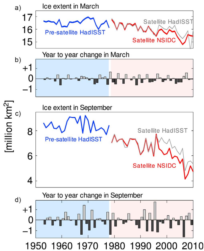
Figure 1. Evolution of Arctic sea-ice extent in (a) March and (c) September and the year-to-year changes in (b) March and (d) September. For this figure, an offset of +0.35 \cdot 10^6 \text{ km}^2 in September and of -0.16 \cdot 10^6 \text{ km}^2 in March has been added to the entire original NSIDC dataset [Fetterer et al. , 2002, 2010] to make the time series consistent with the original HadISST satellite time series during the period 1979–1996 [Met Office Hadley Centre, 2006].
