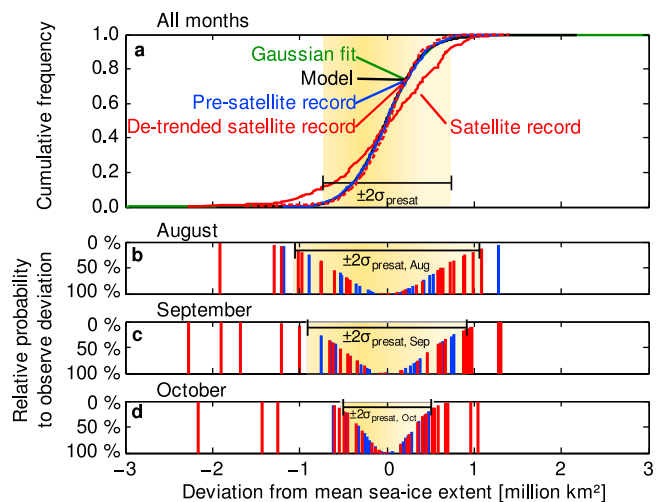
Figure 2. Comparison of the variability of Arctic sea-ice extent. (a) Cumulative frequency of the deviations from the long-term mean as estimated from the pre-satellite record (blue), the model simulation (black), a Gaussian fit to the pre-satellite record (green), the not-detrended satellite record (red solid), and the linearly detrended satellite record (red dashed). (b–d) Deviations from the long term mean of the pre-satellite (red) and satellite (blue) sea-ice extent during August, September and October. The length of the lines is given by one minus the likelihood of observing such deviation. The shaded areas denote plus/minus two standard deviations for that month from the pre-satellite record. Note that in Figures 2b–2d many lines of the pre-satellite record are hidden behind those of the satellite record within the yellow-shaded area.
