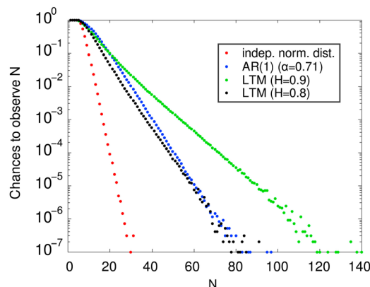
Figure 3. Likelihood to observe a certain number N of consecutive months below the long-term mean in a time series as long as the satellite record for a time series with no memory (red), short-term memory (blue), long-term memory (green and black).
