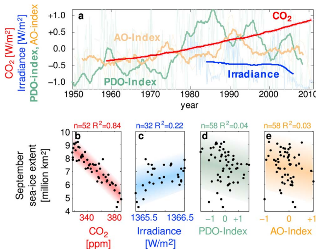
Figure 4. Relationship between sea-ice evolution and various forcings. (a) Temporal evolution of solar irradiance [Fröhlich, 2000], AO-index [Thompson and Wallace, 1998], PDO-index [Mantua and Hare, 2002], and CO 2 concentration (scaling with a 1.66 W/m 2 equivalence for a 100 ppm increase [Intergovernmental Panel on Climate Change, 2007]). The thin lines denote monthly values, while thick lines denote averages over 1 year (CO 2 ), 5 years (AO-index, PDO-index) and 10 years (solar irradiance). (b–e) September sea ice extent from 1953 until 2010 is plotted against annual mean values of the various forcings whenever data was available. The R 2 values are calculated for a standard linear regression as indicated by the shading ( \pm 2\sigma ).
