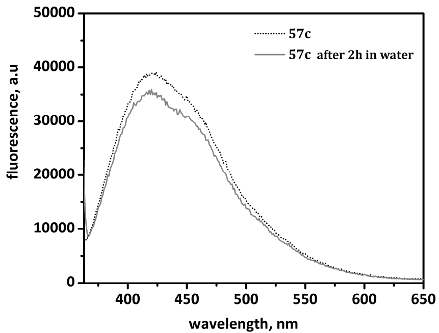
Figure A2. Stability of the spin-coated radical 57c film in aqueous media.
