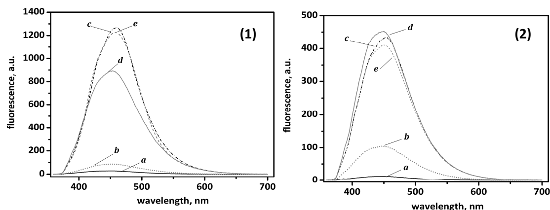
Figure 2.15. Fluorescence spectra of the imino nitroxide 57d in MeOH with the concentration (1) ( 2.5 \times 10^{-5} M), (2) ( 2.5 \times 10^{-6} M) and an excitation wavelength of 346 nm under different conditions: (a) pure solution of the radical; (b) after reaction with \text{CF}_3\text{COOH} ( 1.8 \times 10^{-5} M); (c) after reaction with cysteine ( 5 \times 10^{-4} M); (d) after reaction with ascorbic acid ( 5 \times 10^{-4} M); (e) after sequential reactions with cysteine ( 5 \times 10^{-4} M) and \text{CF}_3\text{COOH} ( 1.8 \times 10^{-5} M).
