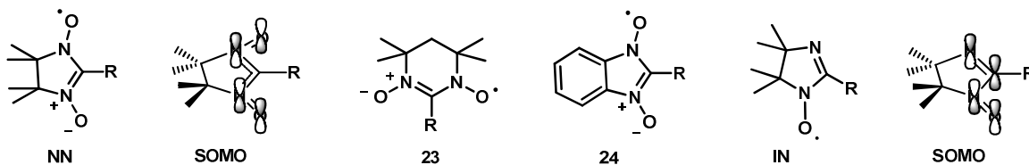
Figure 1.14. Some examples of nitronyl 23 , 24 (NN) and imino nitroxide (IN) radicals, together with the SOMOs of the first and the last cases.
