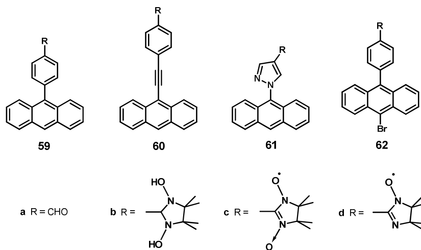
Figure 2.25. Anthracene-based models.
