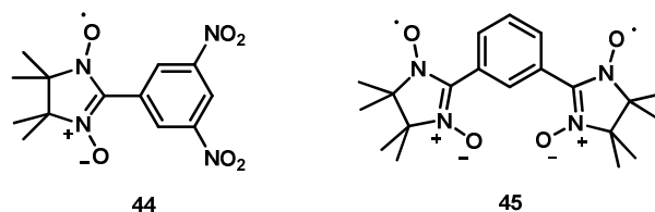
Figure 1.26. Material formed by co-crystallization of two different spin-carrying species: monoradical 44 and biradical 45 .
