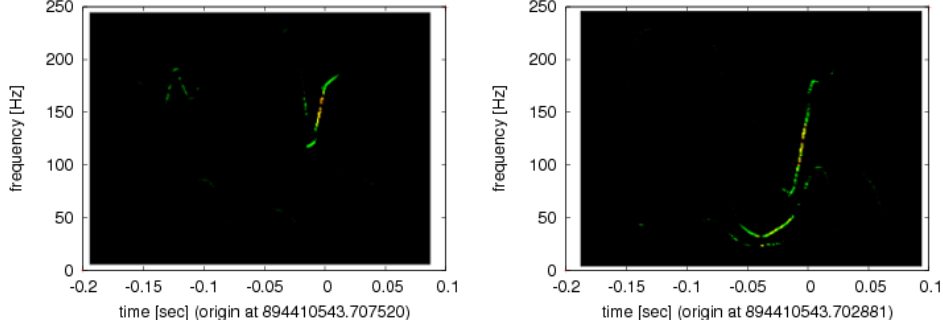
Figure 17. The cluster-enhanced time-frequency maps of the signal injected at GPS time 894410543. H1 is shown in the left panel and L1 in the right panel. We clearly see the burst part of the signal, thus the actual merger. The ringdown and inspiral may be obscured by noise at low SNR.
