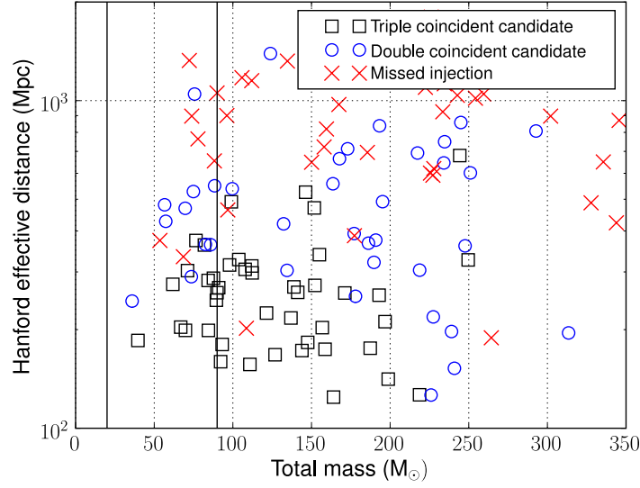
Figure 7. Found and missed injections using TaylorF2 templates terminated at ERD, plotted as a function of the injected effective distance in Hanford and the total mass. The vertical bars mark the limits of the template bank used in the search. For the lower masses, we see that the majority of the closer injections are found in coincidence in all three of the detectors. There is then a band of injections which are found only in two detectors – H1 and L1 and not the less sensitive H2 detector. For higher masses, the results are less meaningful as the template bank was only taken to a total mass of 90M_{\odot} .
