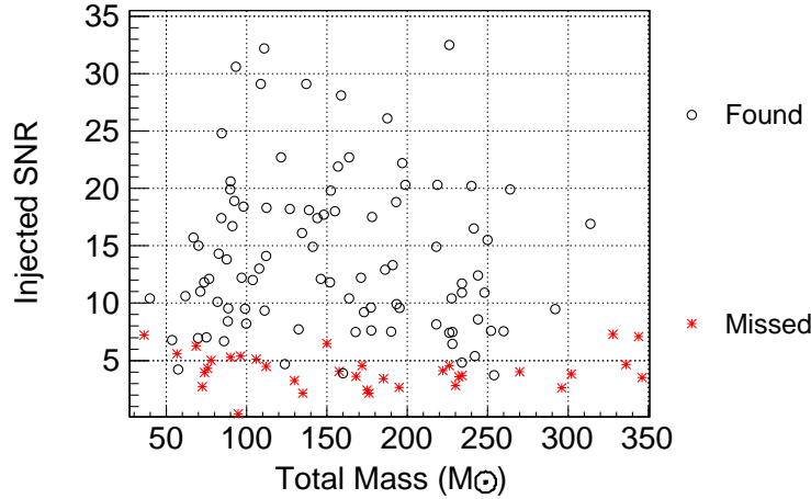
Figure 14. Distribution of injections found by the Q-pipeline in the LIGO Hanford 4 km detector. The total mass of the injected signal is shown on the x -axis and the optimal matched filter signal-to-noise ratio of the injection is shown on the y -axis. Circles show found injections and crosses show missed injections.
