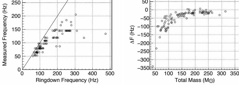
Figure 15. Parameter measurement of signals using the Q-pipeline The left plot shows the measured frequency of the gravitational-wave candidate versus the injected ringdown frequency f_{\text{ring}} computed by equation (12). The right plot shows the difference between Q-pipeline measured frequency and f_{\text{ring}} , against the total mass of the injection.
