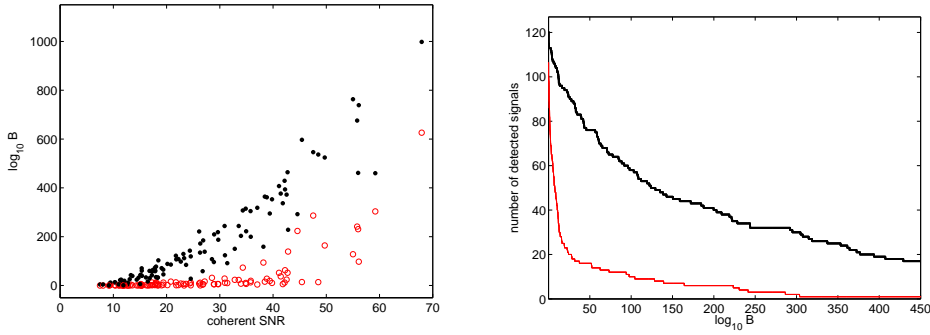
Figure 23. Comparison of the Bayes factors for TaylorF2 and IMRPhenA approximants. Left: The values of the Bayes factors obtained in the analysis of the NINJA data set as a function of the optimal coherent (L1-H1-H2-V1) signal-to-noise ratio at which the signals were injected into instrument noise. The solid (black) dots and the open (red) circles refer to the Bayes factors obtained by using the IMRPhenA and TaylorF2 approximants, respectively. Right: The cumulative number of injections recovered as a function of the Bayes factor. The thin (red) solid line corresponds to the results obtained by using the TaylorF2 approximant, whereas the thick (black) solid line refers to the IMRPhenA approximant. A threshold of \log_{10} B_{SN} = 3 has been used.
