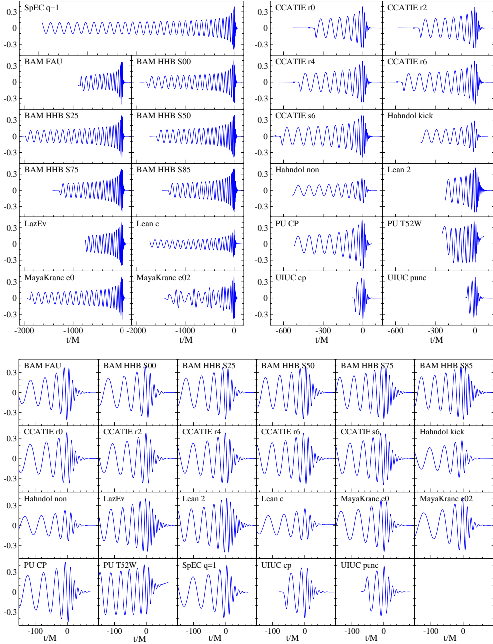
Figure 1. Summary of all submitted numerical waveforms: r/M \text{Re}(h_{22}) The x -axis shows time in units of M and the y -axis shows the real part of the (\ell, m) = (2, 2) component of the dimensionless wave strain rh = rh_+ - irh_\times . The top panels show the complete waveforms: the top-left panel includes waveforms that last more than about 700M , and the top-right panel includes waveforms shorter than about 700M . The bottom panel shows an enlargement of the merger phase for all waveforms.
