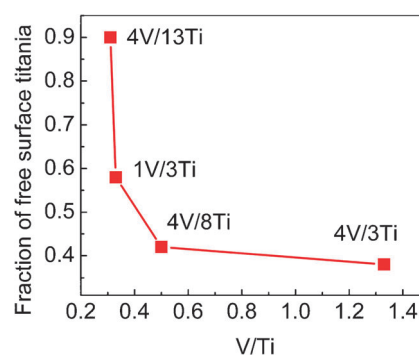
Fig. 6 Fraction of uncovered titania surface as a function of the V/Ti ratio comprising 4V3Ti/SBA-15 (7620), 4V8Ti/SBA-15 (7624), 1V3Ti/SBA-15 (7606), and 4V13Ti/SBA-15 (9954). The free titania surface was estimated from the ratio of the height of the peaks at 2180 \text{cm}^{-1} in the FTIR spectrum of CO adsorbed on the V-containing catalyst and the corresponding support. The peak is attributed to CO adsorbed on coordinatively unsaturated \text{Ti}^{\text{IV}} ions.
