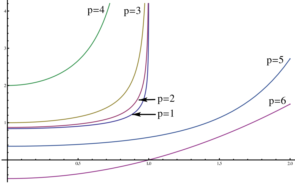
Figure 1: A plot of U vs. r for the solutions (29). We have set R = C_p = 1 ( R = i for p > 4 ). Note that for p > 4 , r diverges toward U = \infty .
