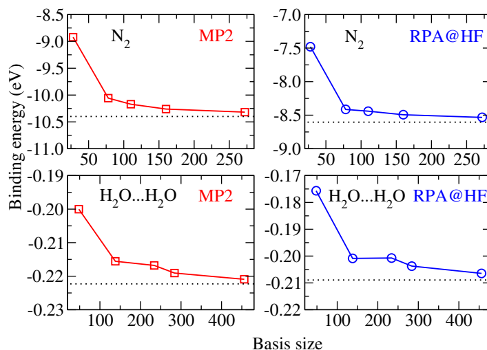
Figure 12. Convergence of BSSE-corrected MP2 and RPA@HF binding energies for \text{N}_2 ( d = 1.1 \text{ \AA} ) and the water dimer (PBE geometry) as a function of the NAO basis set size. The first four points correspond to NAO tier 1 to tier 4 basis sets and the last point corresponds to the composite ‘tier 4 + a5Z-d’ basis. The dotted horizontal line marks the aug-cc-pV6Z results.
