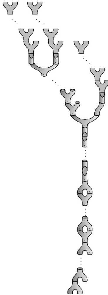
Fig. 1. This figure depicts the normal form of an open–closed cobordism in \mathbf{2Cob}_{\mathbf{O} \rightarrow \mathbf{C}}^{\text{ext}}[\vec{n}, \vec{m}] without precomposition with a permutation, i.e. it shows the open–closed cobordism (3.83).
