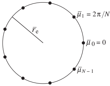
FIG. 1. N point particles of equal mass m in uniform circular motion—the mutual interaction is given by the symmetric potential (half-retarded plus half-advanced potential). We prove that there exists a unique radius \bar{r}_e such that the configuration is in equilibrium.
