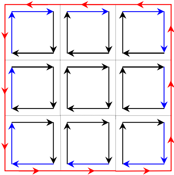
FIG. 5 (color online). A larger parallel transport loop with 12 oriented links on the boundary. As before, the parallel transport matrices along the links appear in pairs and are sequentially integrated over using the uniform measure. The new ingredient in this configuration is an elementary loop at the center not touching the boundary.
