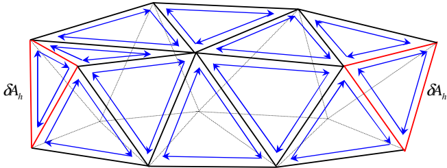
FIG. 6 (color online). Correlations between action contributions on hinge h and hinge h' arise to lowest order in the strong coupling expansions from diagrams describing a narrow tube connecting the two hinges. Here vertices represent points in the dual lattice, with the tubelike closed surface tiled with parallel transport polygons. For each link of the dual lattice, the SO(4) parallel transport matrices \mathbf{R} are represented by an arrow.
