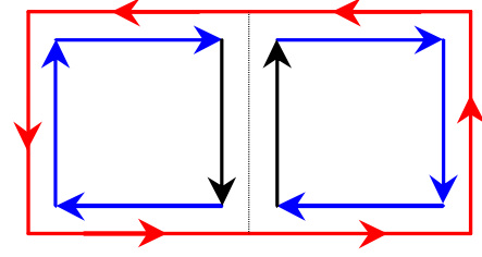
FIG. 4 (color online). A parallel transport loop with six oriented links on the boundary.
