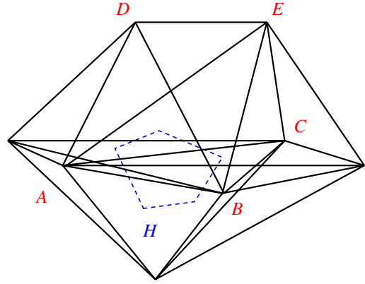
FIG. 1 (color online). Elementary polygonal path around a hinge (triangle) in four dimensions. The hinge ABC , contained in the simplex ABCDE , is encircled by the polygonal path H connecting the surrounding vertices which reside in the dual lattice. One such vertex is contained within the simplex ABCDE .
