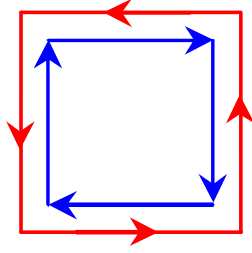
FIG. 3 (color online). A parallel transport loop with four oriented links on the boundary. The parallel transport matrices \mathbf{R} along the links, represented here by arrows, appear in pairs and are sequentially integrated over using the uniform measure.
