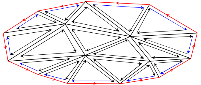
FIG. 2 (color online). Gravitational analog of the Wilson loop. A vector is parallel transported along the larger outer loop. The enclosed minimal surface is tiled with parallel transport polygons, here chosen to be triangles for illustrative purposes. For each link of the dual lattice, the elementary parallel transport matrices R(s, s') are represented by arrows. In spite of the fact that the (Lorentz) matrices \mathbf{R} can fluctuate strongly in accordance with the local geometry, two contiguous, oppositely oriented arrows always give RR^{-1} = 1 .
