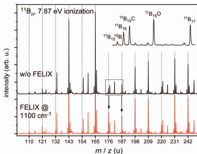
FIG. 1. Mass spectra of B_n clusters obtained by ionization with an F_2 laser ( 157 nm, 7.87 eV) using a target made from isotopically enriched ^{11}\text{B} (99.4%). The mass spectra contain carbide and oxide contaminations. The inset shows the detailed assignment for a selected mass range. At the photon energy of 7.87 eV, the ionization efficiency of the pure boron clusters, as well as the contaminations, is strongly size dependent. The lower trace shows the IR induced enhancement for B_{16} and B_{17} at 1100 \text{cm}^{-1} .
