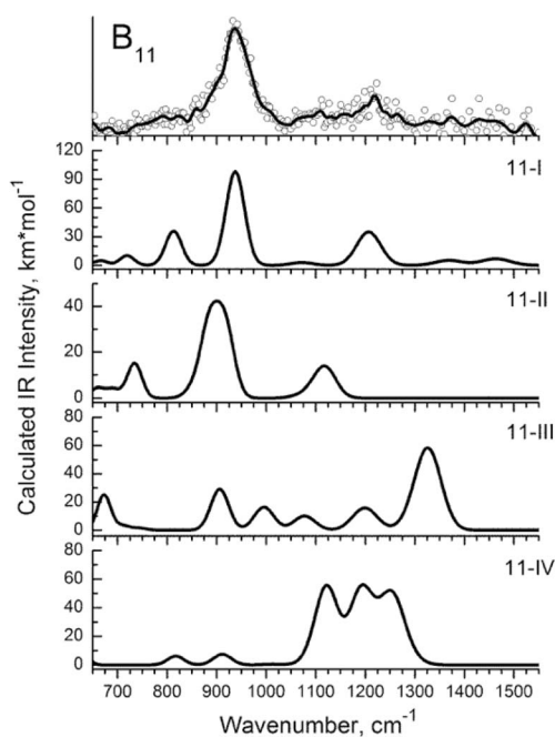
FIG. 2. IR-UV2CI spectrum of B_{11} (top) compared with the IR spectra of low lying isomers from DFT calculation (PBE0/6-311+G(d)). The open circles in the top spectrum correspond to the original data points folded with a 7-point binomial weighted average (solid line). The calculated spectra were generated using Gaussian line widths of 2% of the central wave number.
