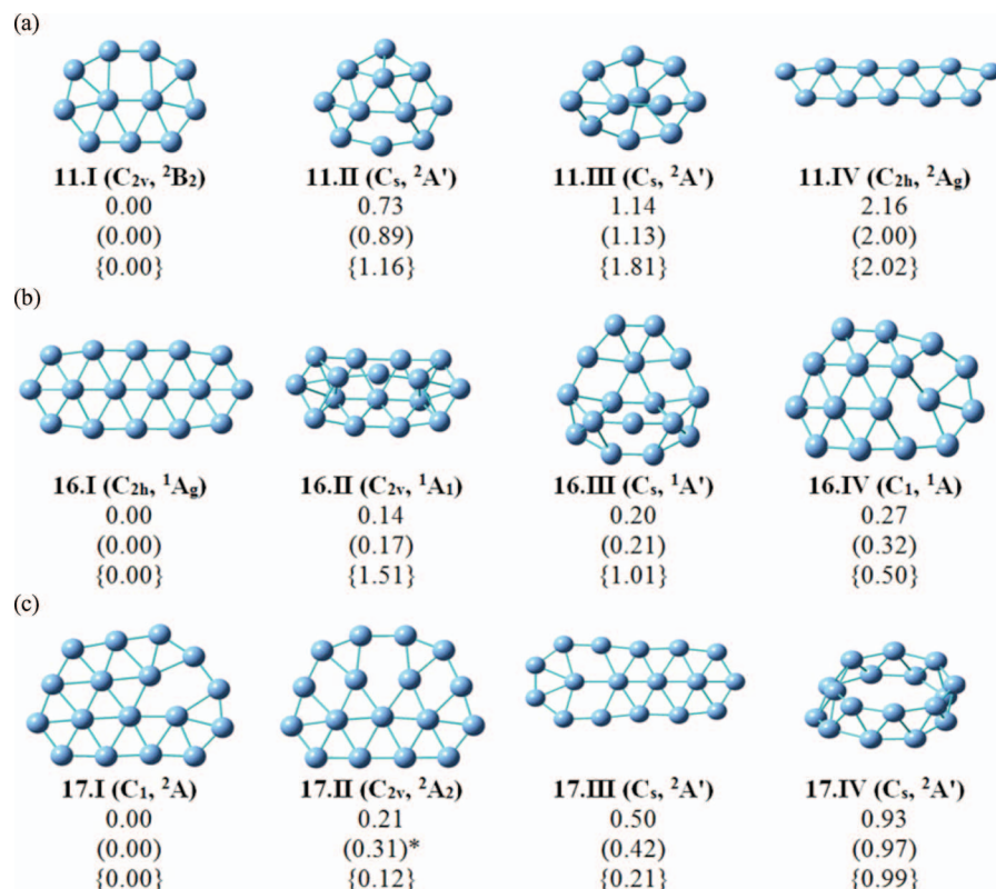
FIG. 5. The global minima and top three low-lying isomers of B 11 (a), B 16 (b), and B 17 (c). Relative energies in eV are given at the PBE0/6-311+G(d) level, TPSS/6-311+G(d) level (in parenthesis), and B3LYP/6-311+G(d) level (curly brackets). All values are corrected for zero-point vibrational energies, except for structure 17-II at the TPSS/6-311+G(d) level of theory, which is a saddle point (see text).
