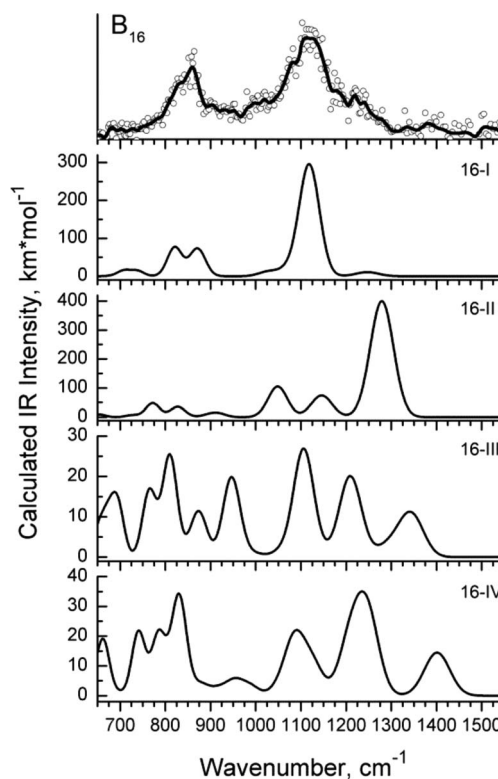
FIG. 3. IR-UV2CI spectrum of B_{16} (top) compared with the predicted IR spectra of low lying isomers at the PBE0/6-311+G(d) level of theory. See the caption of Fig. 2.
