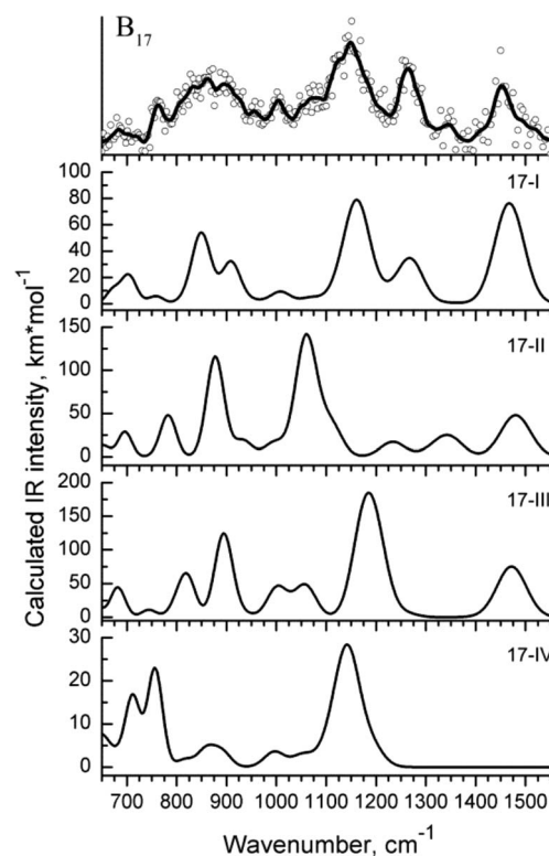
FIG. 4. IR-UV2CI spectrum of B_{17} (top) and comparison with the IR spectra of low lying isomers at the PBE0/6-311+G(d) level of theory. See the caption of Fig. 2.
