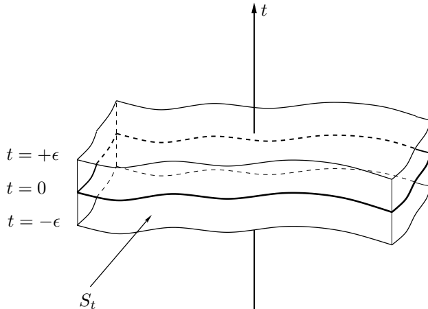
Figure 1: Smearing of the surface S into the third dimension. We obtain an array of surfaces S_t labelled by the parameter t with t \in \{-\epsilon, +\epsilon\} . The original surface S is associated with t = 0 .
