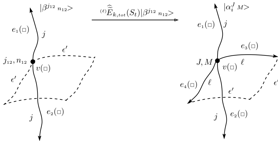
Figure 6: The SNF |\beta^{j12} n_{12} \rangle is transformed into a new SNF |\alpha_i^J M \rangle by the action of {}^{(\ell)}\widehat{E}_{k,tot}(S_t) .
