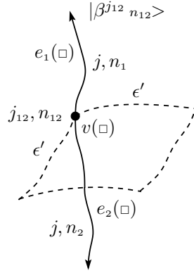
Figure 5: SNF |\beta^{j_{12}} n_{12}\rangle that consists of two edges, whereby one is of type up and the other of type down with respect to the surface S_t . These two edges carry both a spin label j and couple at the vertex v(\square) to an resulting angular momentum j_{12} .
