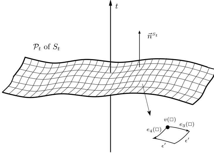
Figure 3: Partition \mathcal{P}_t of the surface S_t into small squares with an parameter edge length \epsilon' .
