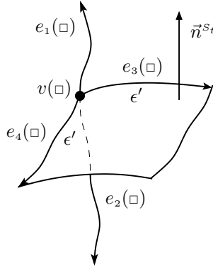
Figure 4: An non-vanishing contribution to \langle T_{s'} | {}^{(\epsilon)}\widehat{E}_k(\square) | T_s \rangle can only be achieved if T_s contains edges of type up and/or down, respectively with respect to the surface S_t . Moreover, the edges e_3(\square), e_4(\square) have to be attached to T_s in this specific way.
