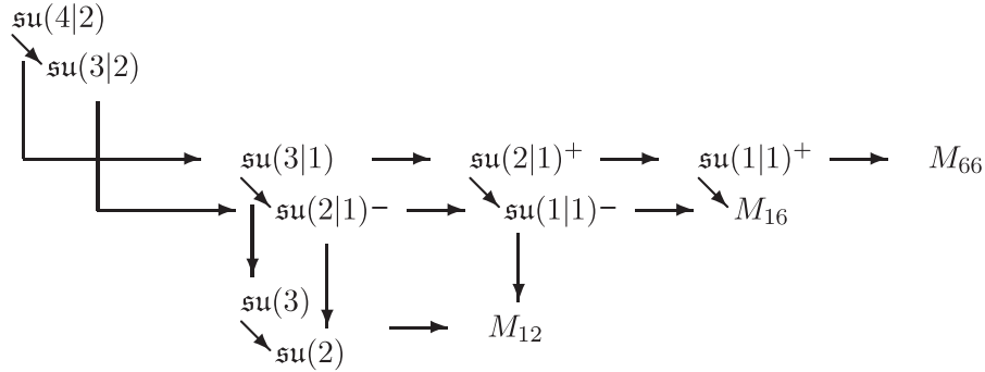
Figure 2. Structure of closed sectors of PWMT. When moving along a vertical/horizontal line, the index range of \alpha/a is reduced by one, i.e. one index value is deactivated. When moving along a diagonal line, one index a is fixed to a particular value.
