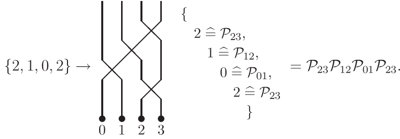
Figure A.1. Graphical representation of the permutation symbol \{2, 1, 0, 2\} .
