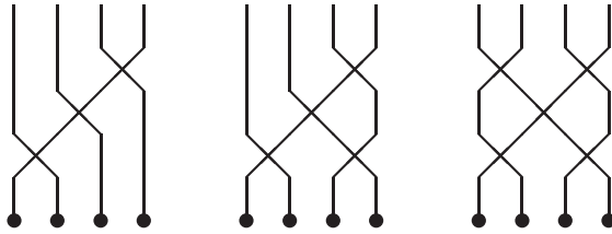
Figure 1. Three planar Feynman diagrams of range R = 4 . The left interaction contains at least 3 four-vertices and appear at three loops, i.e. \mathcal{O}(\lambda^2) . The middle one contains at least 4 four-vertices and can appear only at four loops, i.e. \mathcal{O}(\lambda^3) . The right one may (in principle) represent a fermionic loop and could also arise at four loops.
