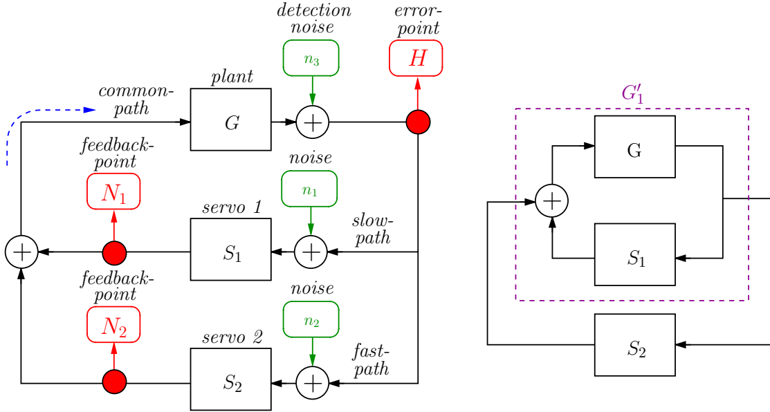
Figure 2.9.: Left: Split-path feedback loop consisting of a plant and two servos. Three independent noise sources are added and signals are recorded by three measurement channels. Signals flow clockwise, as indicated by the dashed arrow. Right: A rearrangement of the loop as a single-path loop consisting of the equivalent gain of the slow-path and the filter for the fast-path.
