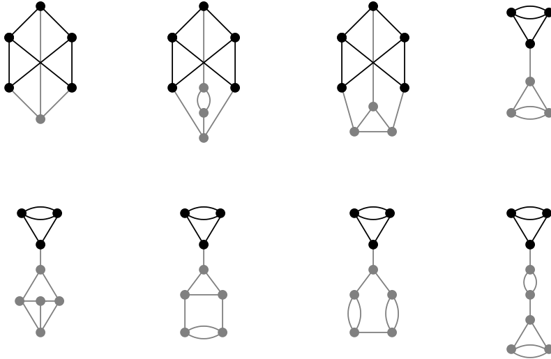
Figure 2: Graphs of parity-even type which vanish identically by virtue of the identities (2.11) and (2.12).
