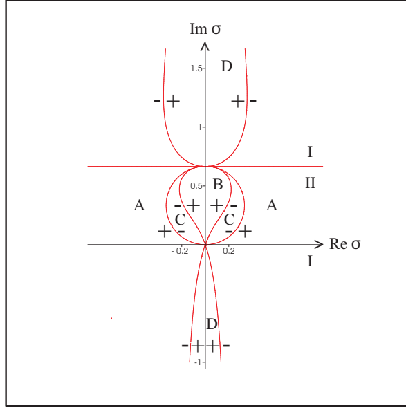
Fig. 1: Sign changes in S for m = 1, M = 1, \Omega = 1, \Lambda = 6 .
