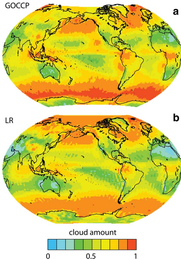
Figure 5. Cloud climatology as seen from space from a downward looking lidar. (a) GOCCP analysis of measurements made by CALIPSO [ Winker et al. , 2010]; (b) LR-AMIP climatology based on the CALIPSO simulator for the period 1980–2005.
