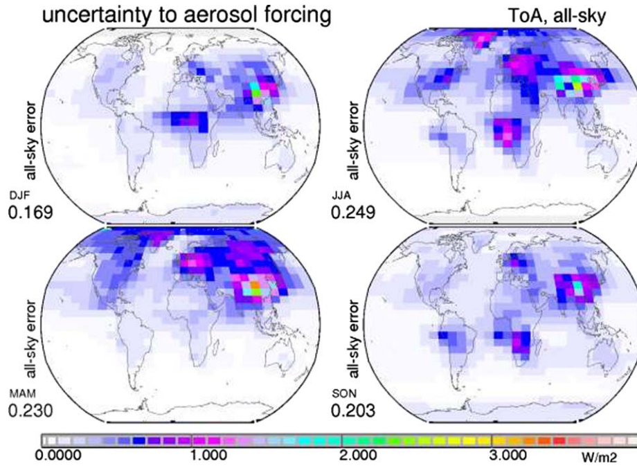
Figure 22. Seasonal maps for estimated uncertainties to current (year 2000) anthropogenic direct aerosol forcing (all-sky, at TOA) of Figure 17 in W/m^2 .
