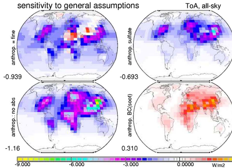
Figure 23. Annual average maps for the anthropogenic aerosol forcing (all-sky, at TOA) for current (year 2000) conditions in W/m^2 , associated with four specific sensitivity scenarios. (top left) The first test applies a simplification, in which the entire fine-mode aerosol is considered to be anthropogenic. (bottom left) The second test has all absorption removed from anthropogenic aerosol. (top right) The third test only considers the sulfate fine-mode anthropogenic impact and (bottom right) the fourth test only considers fine-mode absorbing impacts which are expressed via a BC AOD. Values below the labels indicate resulting direct aerosol forcing global averages.
