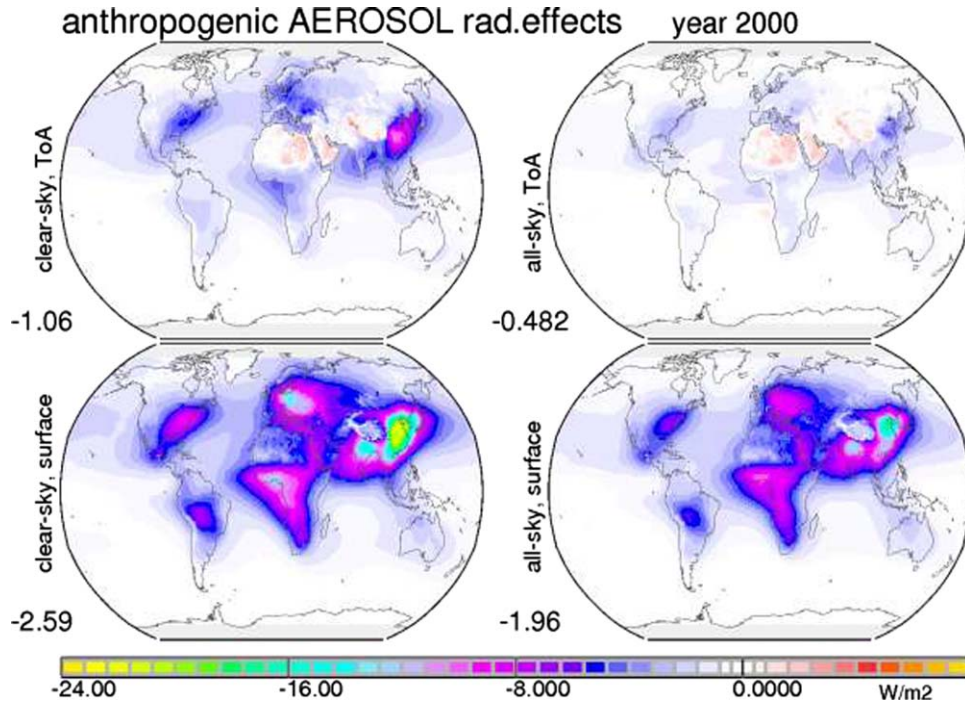
Figure 16. Annual maps for anthropogenic direct aerosol effects at (left column) clear-sky and (right column) all-sky conditions at (top row) TOA and (bottom row) surface in W/m^2 . (Note, all maps are identical to right column data of Figure 14, now at an expanded scale).
