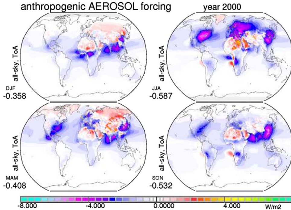
Figure 17. Seasonal maps for the current (year 2000) anthropogenic direct aerosol forcing (= aerosol direct radiative effects under all-sky conditions at TOA) in W/m^2 . Values below the labels display seasonal global averages.
