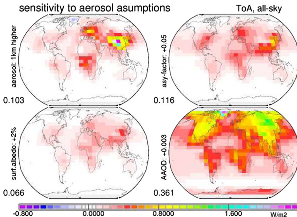
Figure 21. Differences to the annual average anthropogenic aerosol all-sky TOA forcing maps compared to the reference standard simulation in W/m^2 . Four different scenarios were explored: (top left) The aerosol altitude was raised by 1 km, (bottom left) an extra 2% is added to the solar surface albedo, (top right) the fine-mode aerosol size is increased by raising the fine-mode asymmetry-factor by 0.05, and (bottom right) the aerosol absorption is strengthened by adding 0.003 to the AAOD. Values below the labels indicate resulting differences to the standard annual global anthropogenic aerosol forcing of -0.47 W/m^2 .
