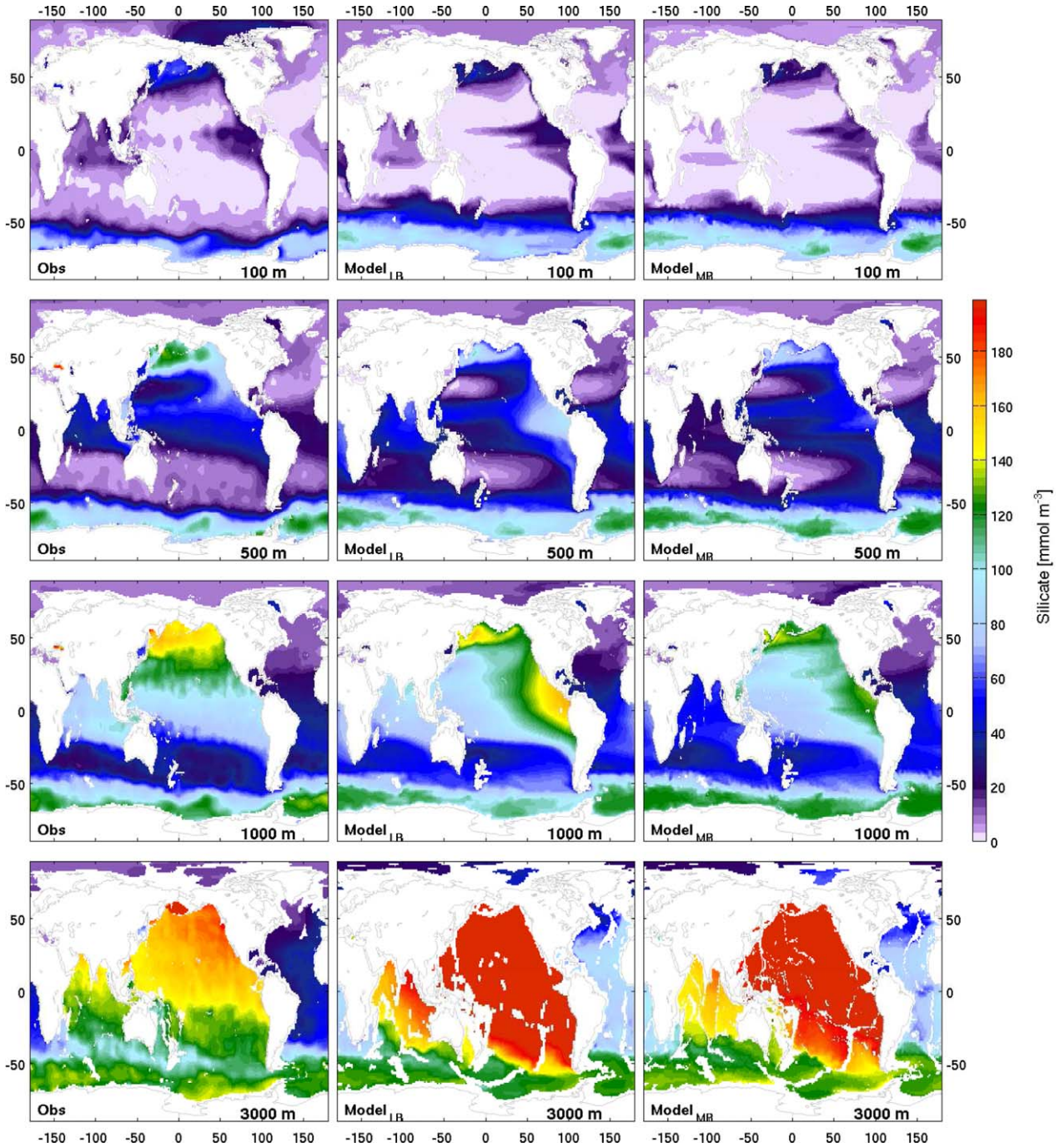
Figure 14. Same as Figure 9 but for silicate. Observations are annual mean fields from WOA.
