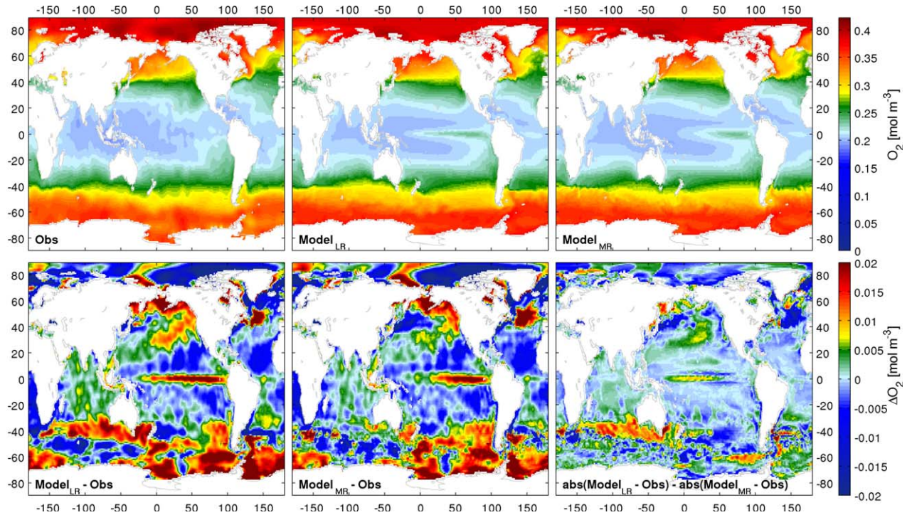
Figure 5. Same as Figure 2 but for surface oxygen. Observations are annual mean fields from WOA.
