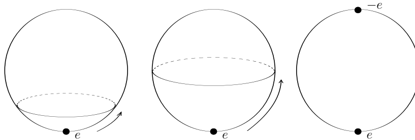
Figure 1: Brane dynamics on S^3 : A stack of D0-branes at e can decay to a D2-brane. Putting more and more D0-branes at e the resulting brane will be localized further and further away from the group unit and eventually the decay product will be a single D0-brane at -e .
