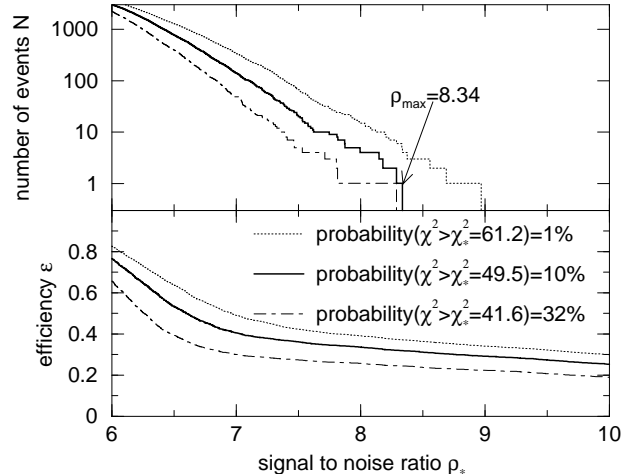
FIG. 2. Top: total number N of events observed, as a function of the SNR threshold \rho_* and the threshold \chi_*^2 . Bottom: fraction \epsilon of Galactic inspiral chirp signals that would lie above SNR threshold \rho_* and below \chi_*^2 threshold \chi_*^2 .
