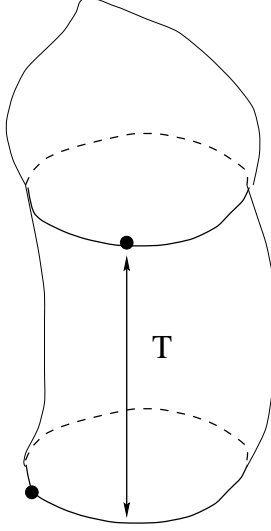
Figure 5: Marking a vertex in the bulk of W_\Lambda(X) . The mark has a distance T from the boundary loop, which itself has one marked vertex.
