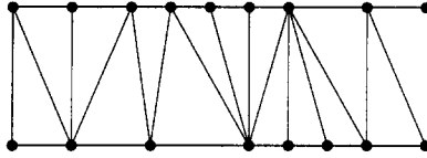
Fig. 1. The propagation of a spatial slice from step t to step t + 1 . The ends of the strip should be joined to form a band with topology S^1 \times [0, 1] .
