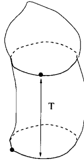
Fig. 5. Marking a vertex in the bulk of W_\Lambda(X) . The mark has a distance T from the boundary loop, which itself has one marked vertex.
