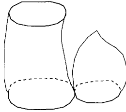
Fig. 4. An alternative representation of the process in Fig. 3: a “baby universe” is created by a global pinching.
