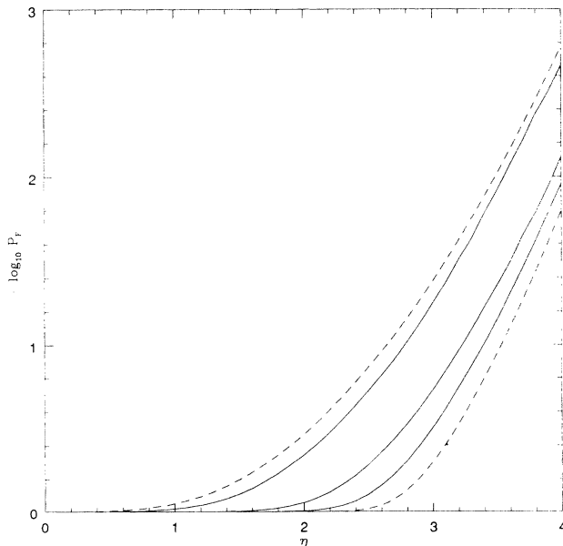
FIG. 4. The figure displays false alarm probability curves where -\log_{10} P_F is plotted vs the threshold \eta for box filters of various bandwidths. There are five curves corresponding to k=2, 3, 10, 32 , and 128 . N=256 for all cases, and the least frequency is n_s=101 for all but the broadband case k=128 . The various curves can be picked out by the property that as k increases they move "down" in the figure implying that the false alarm probability P_F increases for a given value of the threshold. The topmost k=2 and the bottommost k=128 curves are dashed and have been obtained analytically.
