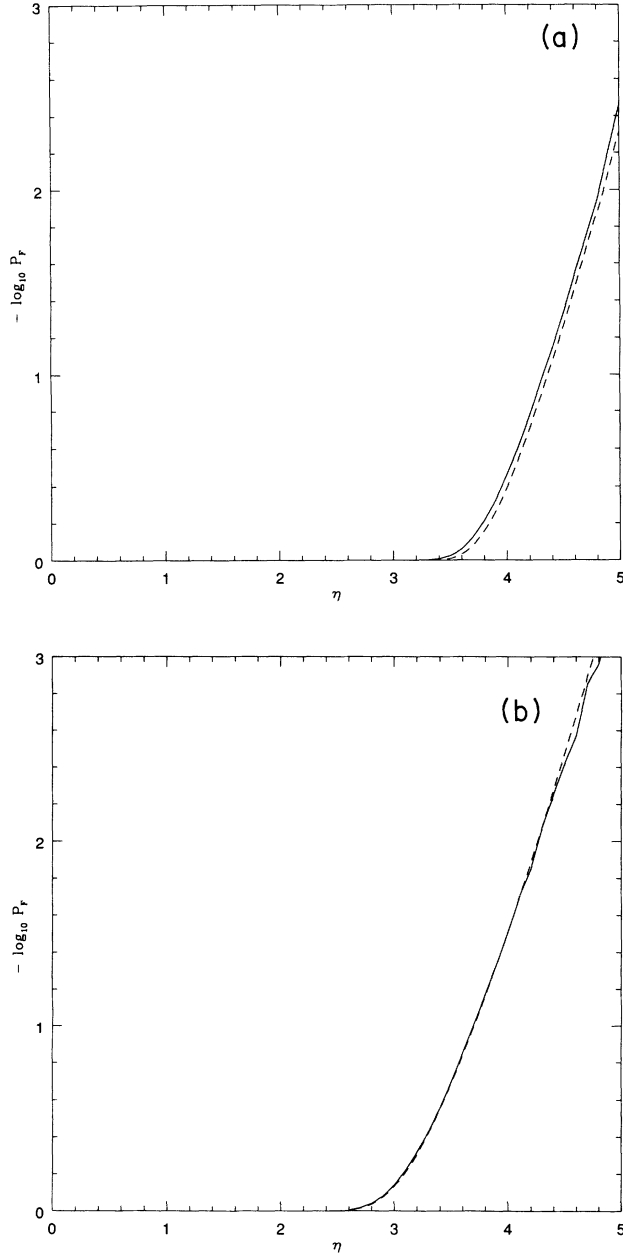
FIG. 5. (a) The figure shows the false alarm probability curve (solid line) -\log_{10}P_F vs the threshold \eta for the chirp with \xi=3 sec, N=8192 , \Delta^{-1}=2.5 kHz, and f_s=100 Hz. The dashed curve is a reference curve for the false alarm probability if all samples are assumed to be independent. The threshold is seen to be slightly lowered by about 0.05. (b) The figure shows the false alarm probability curve (solid line) with the same parameters as in 4 (a) but for the resampled output. The resampling rate is 150 Hz, 1.5 times the seismic cutoff frequency. Since N=8192 the optimal number of samples is N_{\text{eff}}=491 . We observe that this curve coincides with the reference (dashed) curve drawn for N_{\text{eff}} independent samples.
