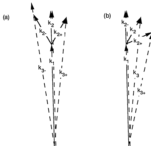
Fig. 2. Wave vectors showing the phase matching for dispersively compensated SFM scheme with central component of the 707-nm beam (a) collinear and (b) non-collinear with the 266-nm beam. The 1, 2, and 3 indices of the k vectors refer to the central wavelengths of 266, 707, and 193 nm, respectively. The plus and minus, if present, indicate that the given vector belongs to a wavelength that is slightly larger or smaller than the central wavelength.
