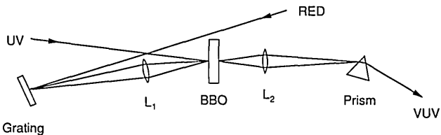
Fig. 1. Experimental arrangement for dispersively compensated SFM of broadband, ultrashort pulses.
