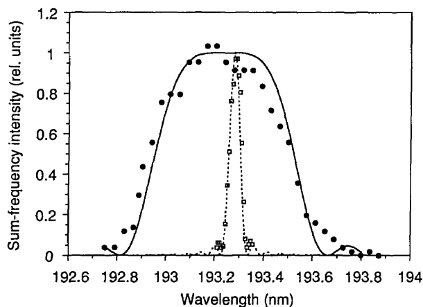
Fig. 3. Measured and calculated SFM spectral acceptance of a 1-mm-thick BBO crystal, uncompensated (squares and dashed curve) and compensated (circles and solid curve).
