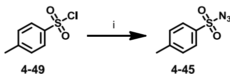
Scheme 4-15: Synthesis of 4-methylbenzenesulfonyl azide ( 4-45 ). Conditions: i NaN 3 , acetone, H 2 O, 0°C, 94%.
