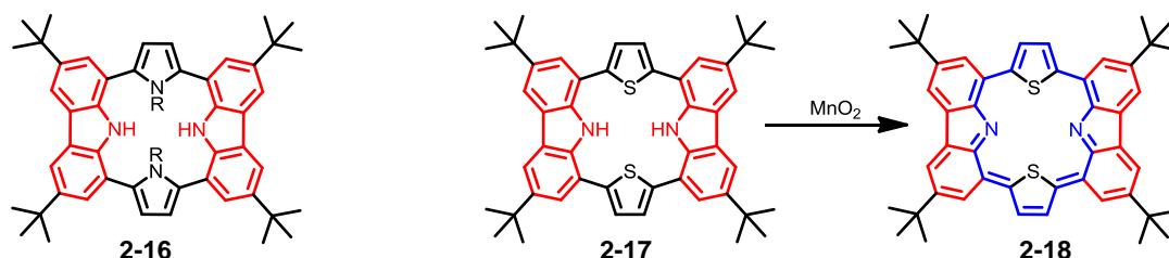
Figure 2-9: Carbazole-containing porphyrinoids 2-16 and 2-17 and core-modified porphyrin 2-18 . [35]
