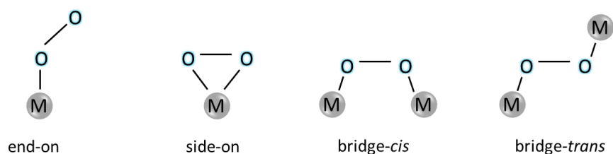
Figure 2-15: Different configuration for molecular oxygen when it interacts with the active sites.
