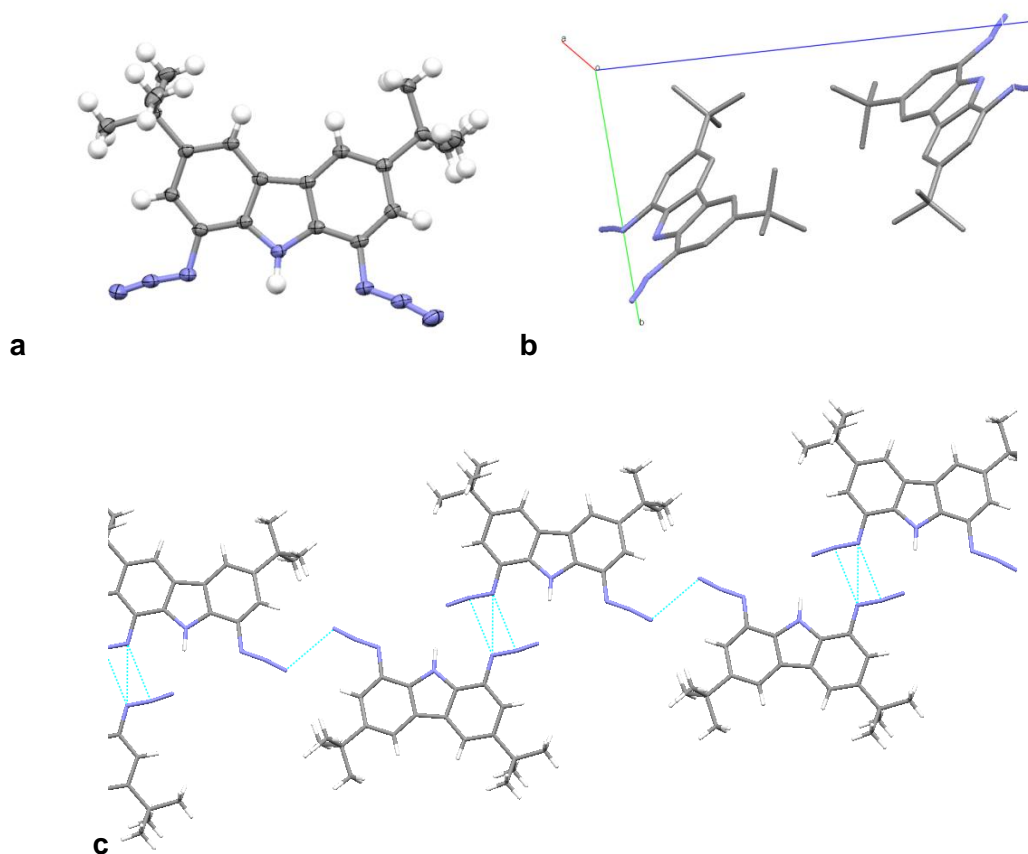
Figure 4-51: Crystal structure of 1,8-diazo-3,6-di- tert -butyl-9 H -carbazole 4-46 a : single molecule (the ellipsoids correspond to 50% probability); b : unit cell (hydrogen atoms are omitted for clarity); c : molecular packing.
