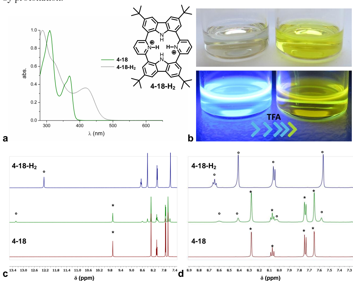
Figure 4-10: a: Electronic absorption spectra of macrocycle 4-18 (in DCM, green) and its dication 4-18-H 2 (in DCM + 1% TFA, dotted line); b: color change upon addition of TFA in ambient light and \lambda = 366 nm; c and d: aromatic region of 1 H NMR spectra of macrocycle 4-18 ( c = 10^{-3} M, CD 2 Cl 2 , 298 K, red,*), its dication 4-18-H 2 (CD 2 Cl 2 + 2 \mu l TFA-d 1 , 298 K, blue,°) and the intermediate state (CD 2 Cl 2 + 1 \mu l TFA-d 1 , 298 K, green)
