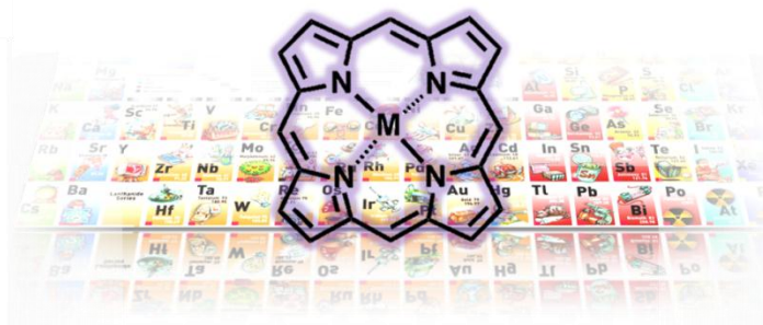
Figure 2-3: Metalloporphyrin.
