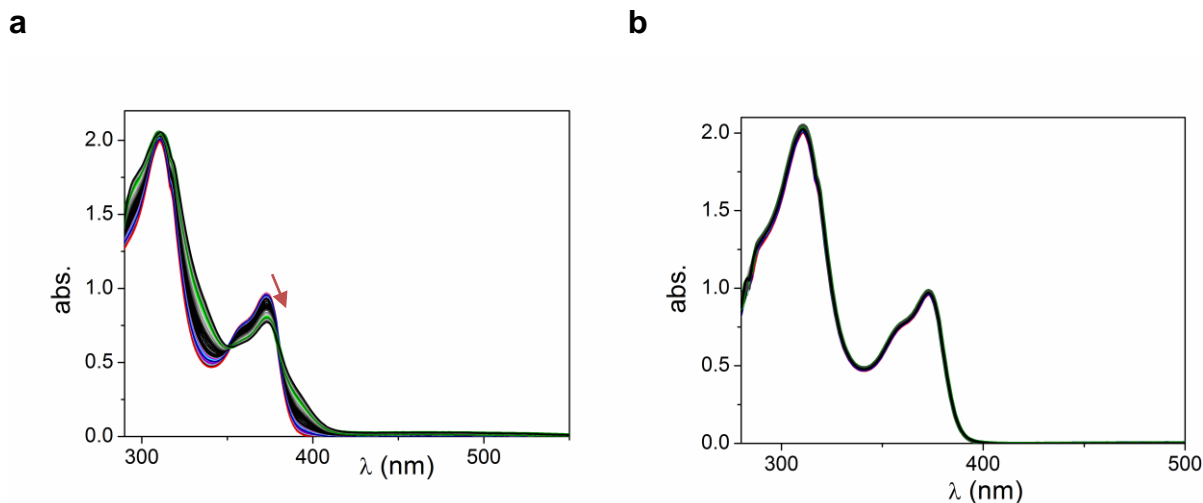
Figure 4-61: Electronic absorption spectra in THF of macrocycle 4-18 ( 5 \times 10^{-5} M) upon titration of a : TBAF and b : TBACl.
