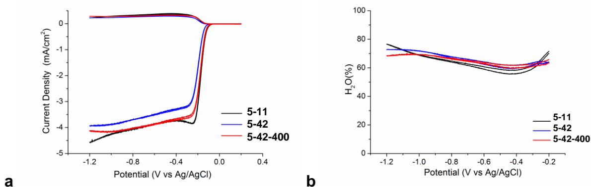
Figure 5-23: a : Ring-disk voltammograms and b : efficiency of \text{H}_2\text{O} production (plotted till -0.2 \text{ V} ) of cobalt complex 5-42 (blue), 5-42-400 (red) benchmark against 5-11 (black) in alkaline conditions ( 0.1 \text{ M KOH} , 1600 \text{ rpm} ).
