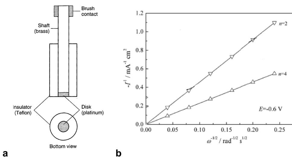
Figure 2-17: a: Schematic illustration of RDE, [129] b: Koutecky–Levich plots at -0.6 V for the theoretical slopes calculated assuming the 2- and 4-electron processes for the \text{O}_2 reduction. [130]
