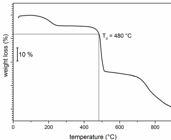
Figure 4-26: TGA of cobalt(II) complex 4-19 under \text{N}_2 atmosphere. 25-900°C, scan rate 10 \text{Kmin}^{-1} .
