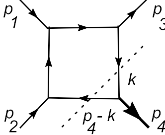
Figure 6: The box diagram corresponding to the integral (B.9)
