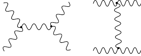
Figure 2: Tree-level diagrams for the color-ordered MHV amplitudes
