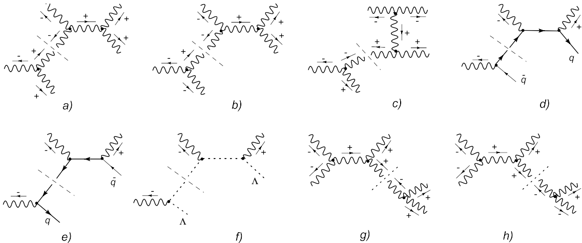
Figure 5: The initial and final particle splitting diagrams: a) the initial MHV amplitude, b)-c) the initial anti-MHV amplitudes, d)-f) the initial matter amplitudes, g)-h) the final MHV and anti-MHV amplitudes. Permutations are not shown.
