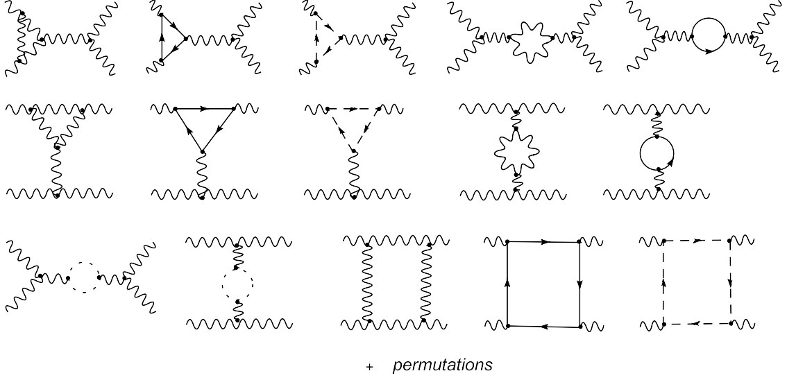
Figure 3: The one-loop diagrams for the color-ordered MHV amplitude in the \mathcal{N} = 4 SYM theory. Particles running inside the loop include all the members of the \mathcal{N} = 4 supermultiplet. The solid and dashed lines correspond to the fermion and scalar particles, respectively.
