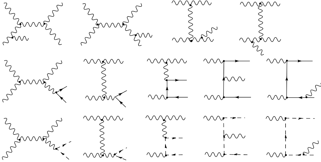
Figure 4: The tree diagrams with three outgoing particles for the color-ordered amplitudes. Permutations are not shown.
