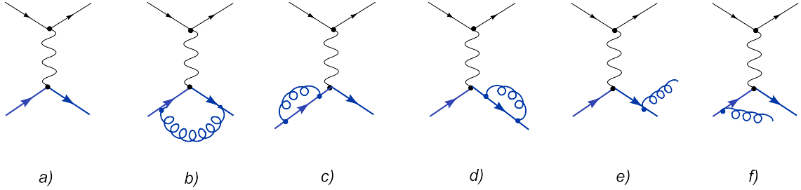
Figure 1: The process of electron-quark scattering in the first order in \alpha_s : a) the Born diagram, b)-d) the corrections due to the virtual gluons, e)-f) the corrections due to the real gluons
