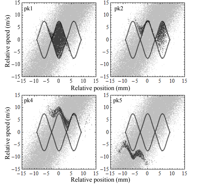
FIG. 3: Light points: longitudinal positions and speeds of simulated molecules at the moment when the decelerator is turned on. Dark points: those molecules that produce the labelled peaks in Fig. 2. Bold lines: region that encloses the trapped molecules (the separatrix), calculated analytically.
