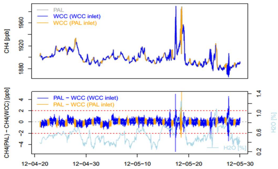
Fig. 19. Same as Fig. 16 for CH 4 .
