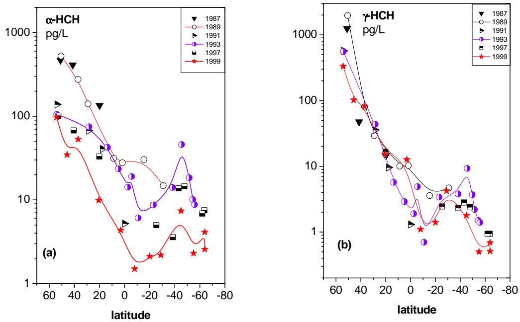
Fig. 3: Measured time trend of \alpha -HCH and \gamma -HCH in the Atlantic Ocean 1987-1999
