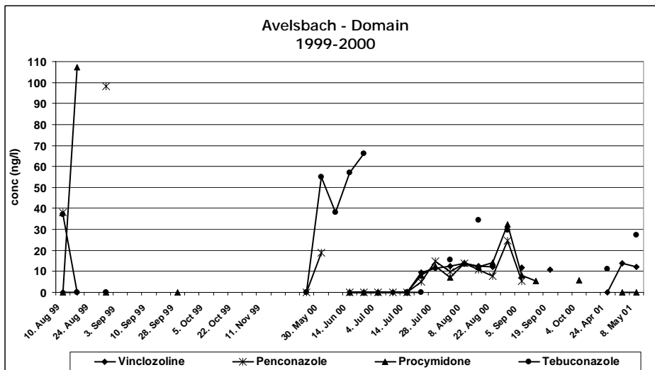
Fig. 4: Fungicide concentrations in a rural site (vineyard).
