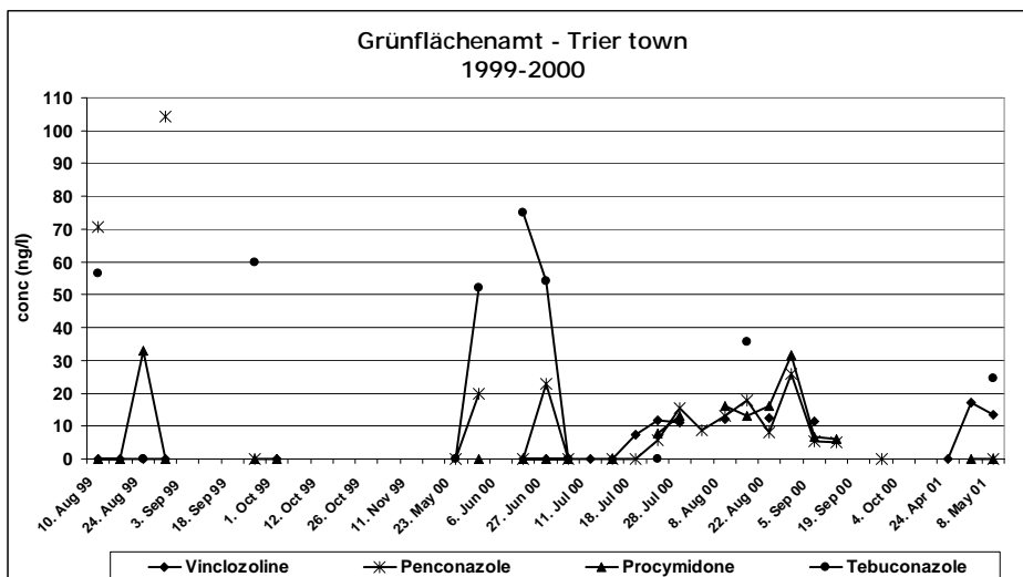
Fig. 5: Fungicide concentrations in an urban site.
