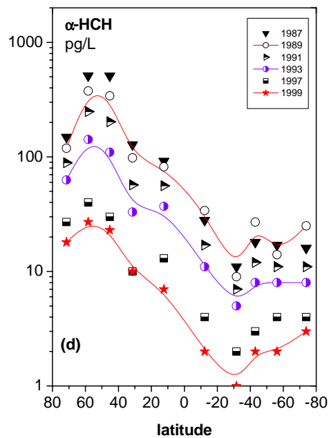
Fig. 4: Model calculation of \alpha -HCH seawater concentration (Li et al., 1996; Wania et al., 1999)
