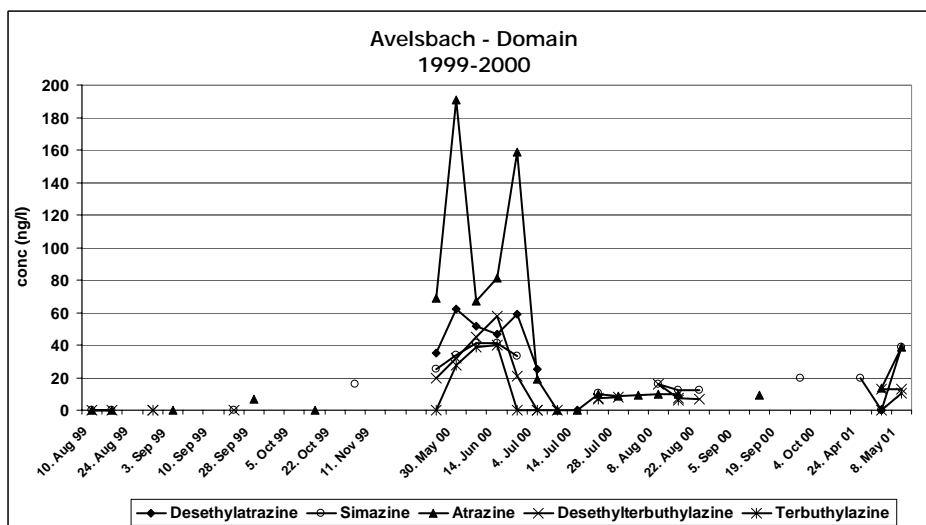
Fig. 2: Herbicide concentrations in an urban site.
