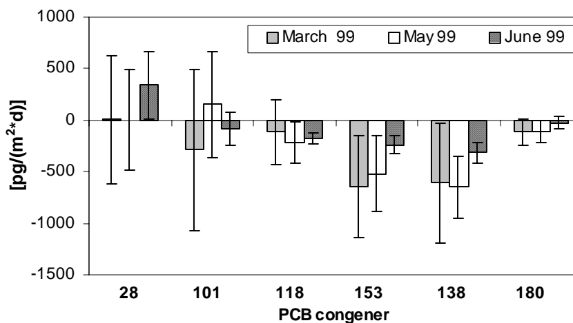
Fig. 3: Net flux of selected PCB congeners for March, May and June calculated with Henry's law constants and enthalpies from Dunnivant et al. (1992) and Burkhard et al. (1985). The arithmetic means and standard deviations are shown.
