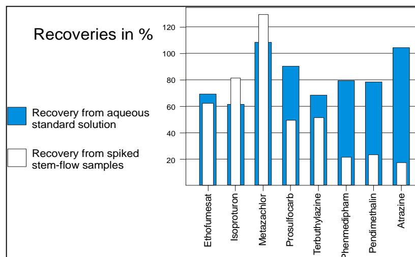
Fig. 2: comparison of recoveries for several substances from aqueous standard solution and stemflow-samples
