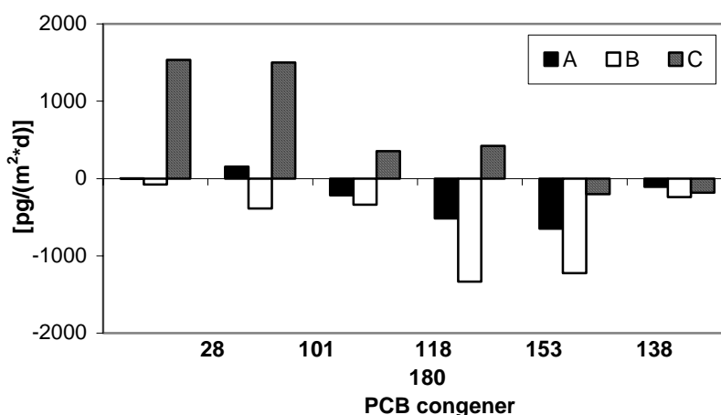
Fig. 2: Net flux of selected PCB congeners for May 1999 calculated with three different sets of HLCs and enthalpies: A) Dunnivant et al. (1992) and Burkhard et al. (1985), B) Brunner et al. (1990) and ten Hulscher et al. (1992), C) Bamford et al. (2000). The arithmetic means are shown.
