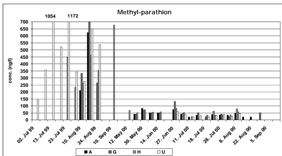
Fig. 7: Methyl parathion concentrations detected in four sampling sites (A = Avelsbach, G = Grünflächenamt Trier town, H = Hospital Geozentrum, U = Universität; cf. Table 1).
