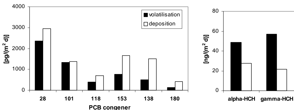
Fig. 1: Volatilisation and deposition fluxes of selected PCB congeners and \alpha - and \gamma -HCH calculated for one sampling pair from May 1999. The Henry's law constants and enthalpies of phase change were taken from Dunnivant et al. (1992) and Burkhard et al. (1985), respectively, for the PCBs and from Kucklick et al. (1991) for the HCHs.
