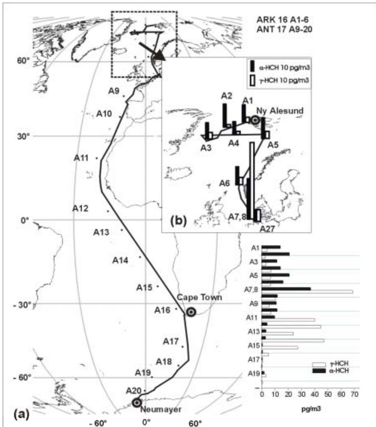
Fig. 1: HCHs in air 1999/2000
