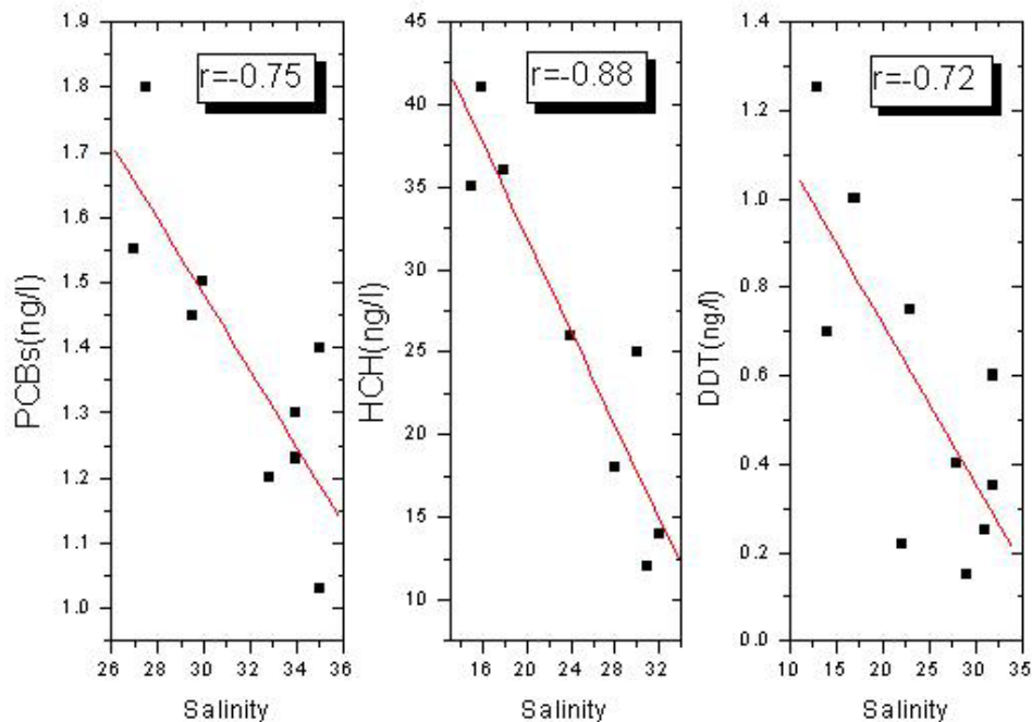
Fig. 2: The relationship between POPs contents in water and salinity in Changjiang estuary in Summer (from Ye et al., 1991)
