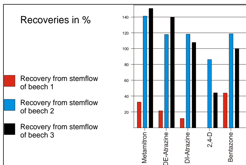
Fig. 1: Variation of recoveries of some selected pesticides from three different stemflow-samples
