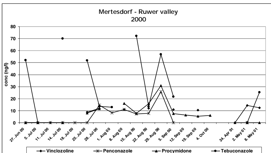
Fig. 6: Fungicide concentrations in a countryside site.
