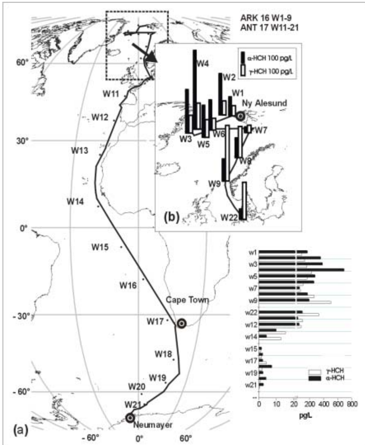
Fig. 2: HCHs in water 1999/2000
