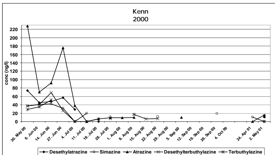
Fig. 3: Herbicide concentrations in an industrial site.
