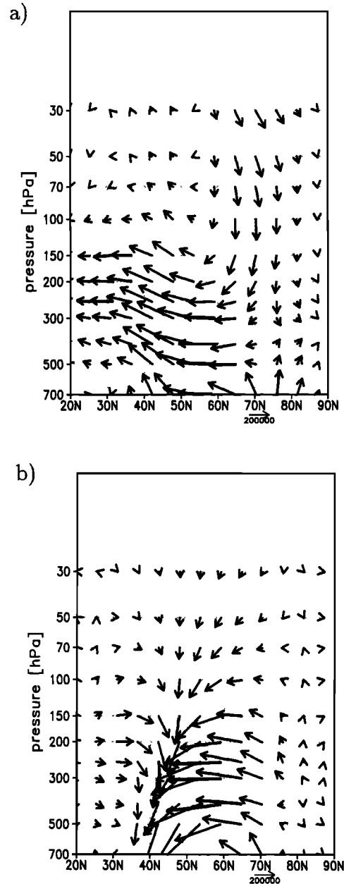
Figure 2. Meridional cross section of difference vectors between the composites of the Eliassen-Palm (E-P) flux (strong minus weak polar vortex state) for (a) zonal wave number (ZWN) 1 and (b) ZWN 2. The arrow scale amounts to 2.0 \times 10^5 \text{ kg s}^{-1} . The vertical scaling factor c is 125.
