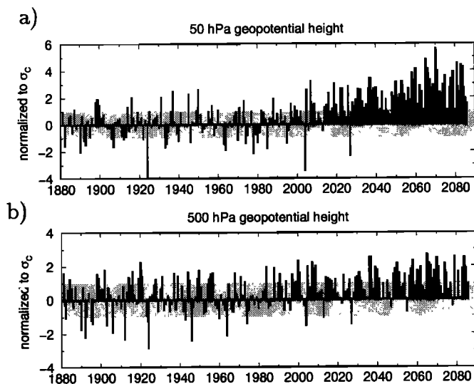
Figure 7. Time series of projections of response pattern, determined from a transient greenhouse gas (GHG) forcing experiment, onto the singular patterns of leading atmospheric circulation mode, determined from the 1900-year control run. The time series for (a) 50-hPa geopotential height field (north of 20°N) and (b) 500-hPa geopotential height field (north of 20°N) are normalized by the standard deviation \sigma_C of the individual projections of the control run.
