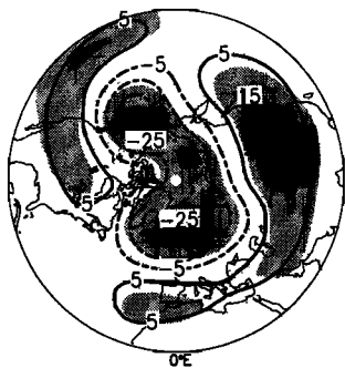
Figure 8. The 500-hPa heterogeneous regression patterns of SVD analysis between 50- and 500-hPa geopotential heights for the GHG experiment on the basis of the time period 2014–2084 of the simulation. The shading corresponds to Figure 4.
