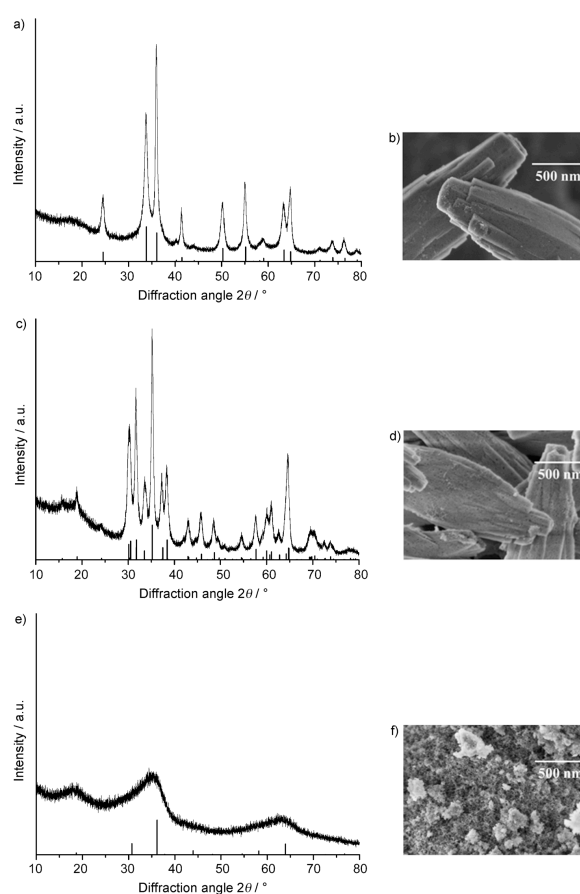
Figure 1. XRD and SEM of calcined samples. The histograms in (a), (c) and (e) represent α-Ga 2 O 3 , β-Ga 2 O 3 and γ-Ga 2 O 3 with ICSD Nr. 27431, 83645 and 152085, respectively. The differences in relative peak intensities between the experimental and literature data in a) can be explained with preferred orientation of the anisotropic crystallites.
