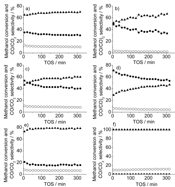
Figure 8. Methanol conversion (●) and CO (Δ), CO 2 : (•) selectivity in the MSR reaction with a) Pd 2 Ga/α-Ga 2 O 3 , b) Pd 5 Ga 3 /α-Ga 2 O 3 , c) Pd 2 Ga/β-Ga 2 O 3 and d) Pd 2 Ga,Pd 5 Ga 3 /β-Ga 2 O 3 , e) Ga-Pd/g-Ga 2 O 3 reduced at 160 °C, and f) a Pd/Al 2 O 3 reference.
