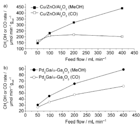
Figure 10. Flow rate variation studies on a) a Cu/ZnO/Al 2 O 3 reference catalyst and b) Pd 2 Ga/ \alpha -Ga 2 O 3 .
