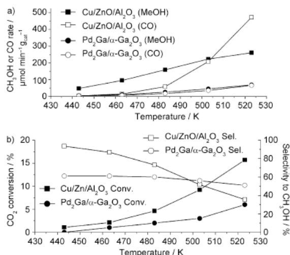
Figure 9. a) Methanol synthesis rates and b) selectivities of Pd 2 Ga/ \alpha -Ga 2 O 3 (●) and a Cu/ZnO/Al 2 O 3 reference catalyst (■).
