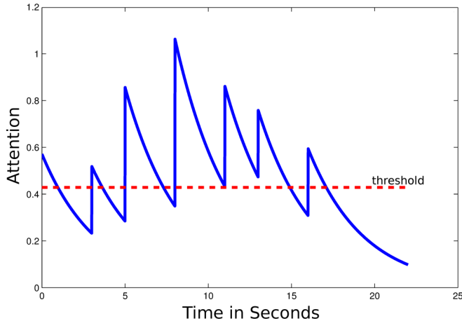
Fig. 2: Exemplar attention function, after applying exponential decay with \alpha = 0.3 on a sequence of \delta spikes. The attention at t = 0 reflects the initial interest at the start of the trial. The horizontal line represents a threshold with \theta = 0.42 .
