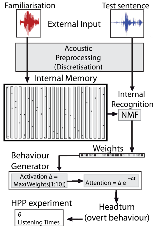
Fig. 1: The Headturn Preference Procedure model, with processing stages and flow of information from top (external input) to bottom (overt behaviour in an experimental setting).
