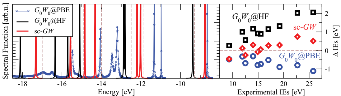
FIG. 3. (Color online) Left: The spectral function of benzene calculated with a Tier 2 basis set. Vertical dashed lines are located at experimental vertical ionization energies from Ref. 46. Right: Comparison of experimental (Ref. 46) and theoretical vertical ionization energies (VIEs) extracted from the spectral function of benzene for sc-GW , G_0W_0@HF , and G_0W_0@PBE .
