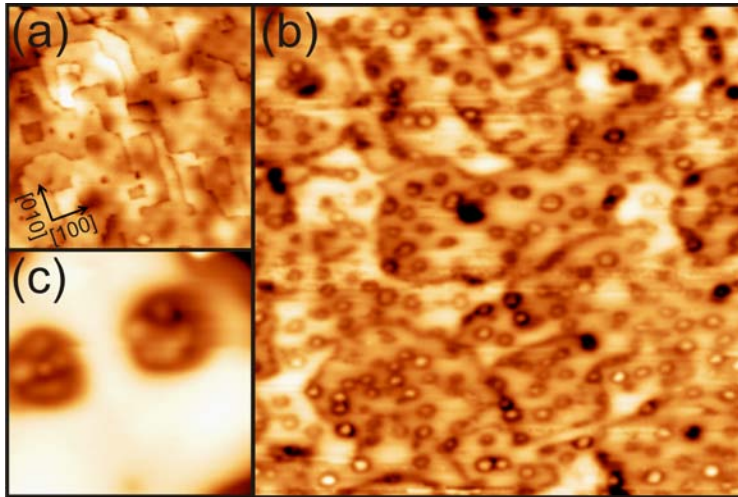
Figure 1: (a) STM topographic image of a bare 10 ML thick MgO film on Mo(001) ( 100 \times 100 \text{ nm}^2 ). (b) Image of \text{Eu}_2\text{O}_3 nano-islands produced by depositing 0.5 ML Eu onto MgO and annealing in \text{O}_2 ( 100 \times 100 \text{ nm}^2 ). (c) Close-up of two \text{Eu}_2\text{O}_3 islands located on an MgO terrace ( 15 \times 15 \text{ nm}^2 ).
